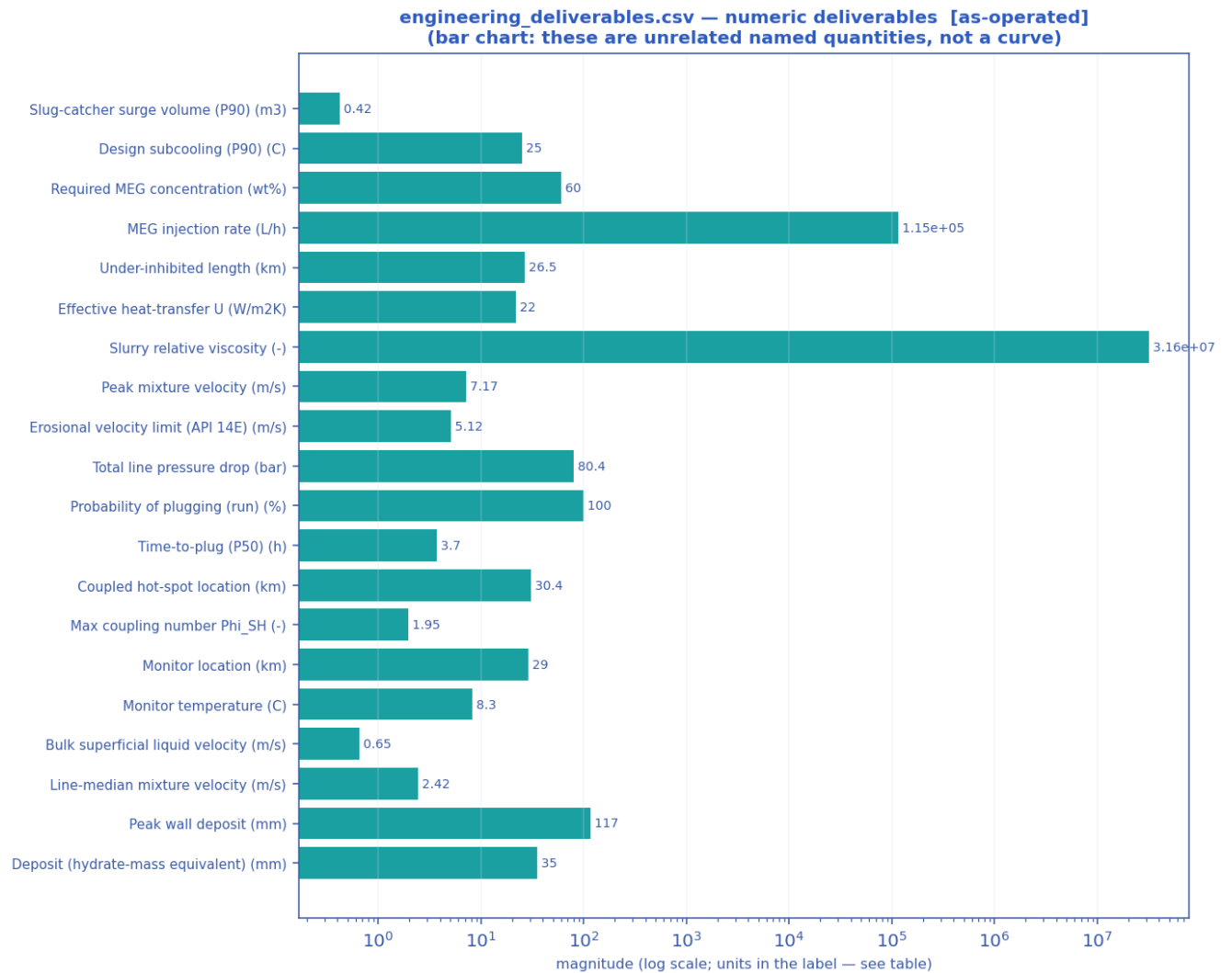
Numeric engineering deliverables as a magnitude chart [as-operated].
