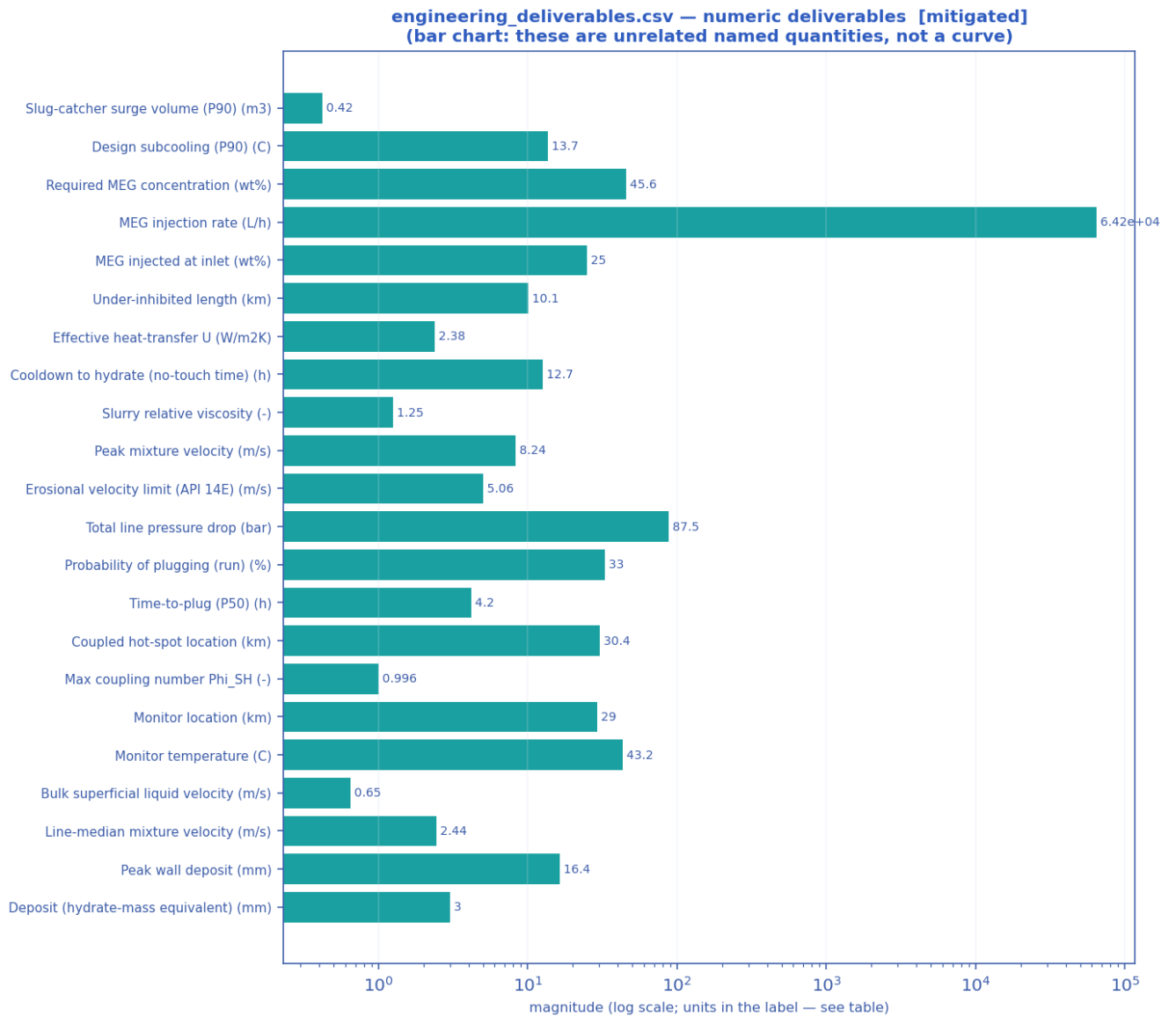
Numeric engineering deliverables as a magnitude chart [mitigated].
