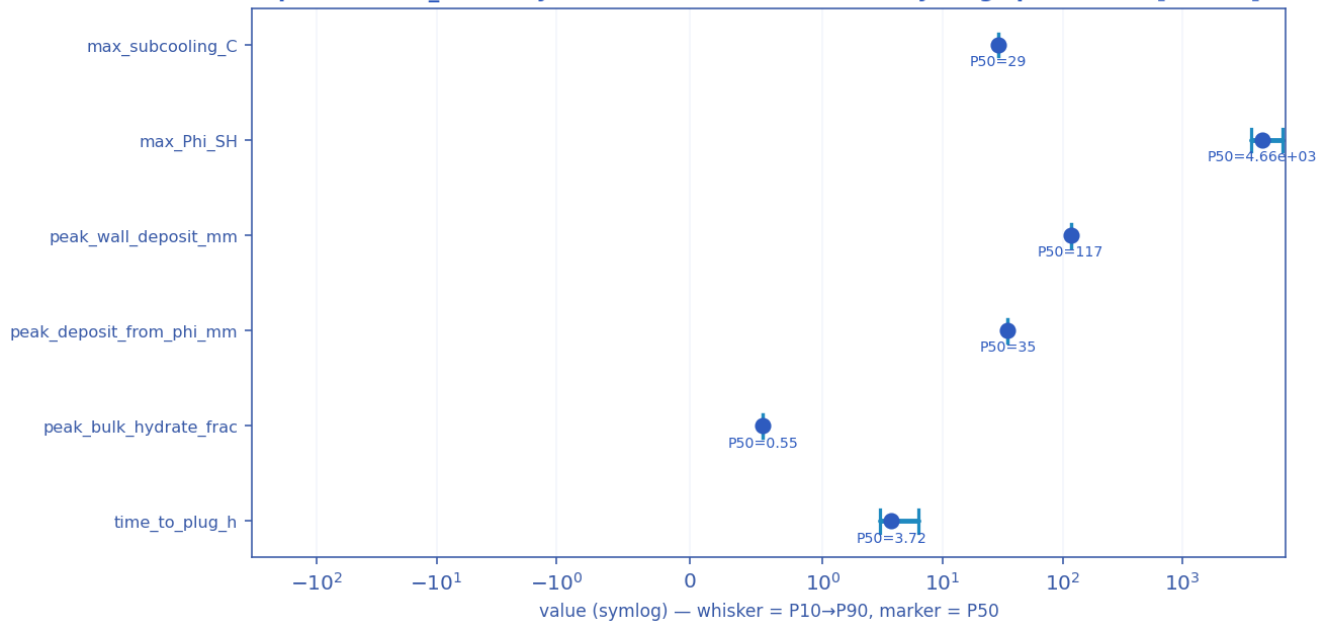
probabilistic_summary.csv — P10/P50/P90 uncertainty range per metric [shut-in]
