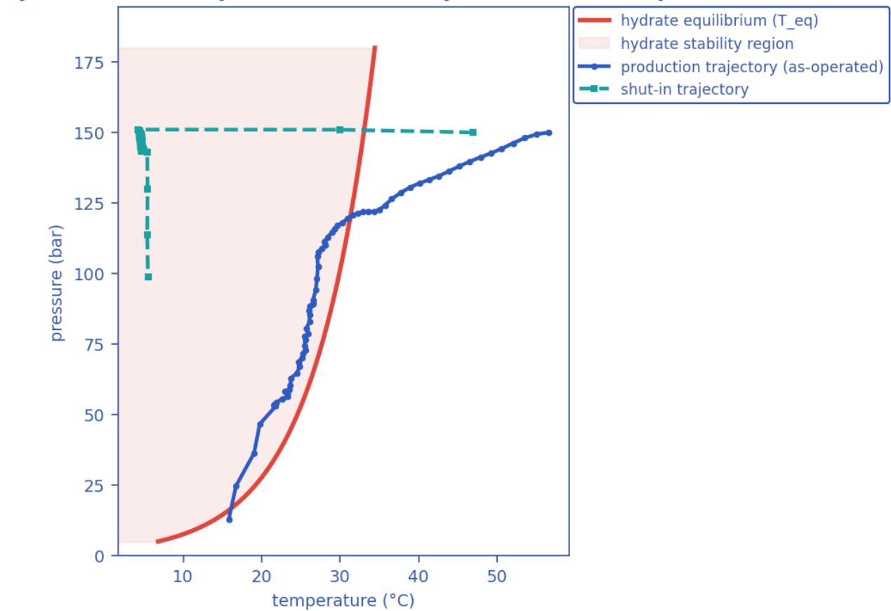
Hydrate-formation prediction: production AND shut-in P–T trajectories overlaid on the hydrate envelope. [as-operated]
