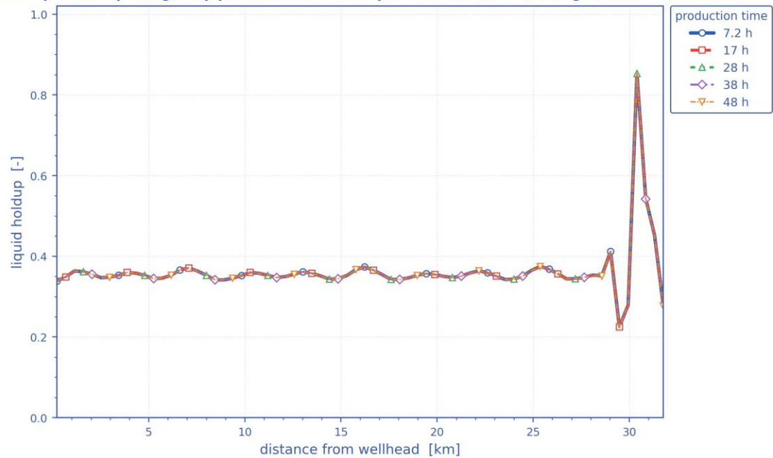
Distribution of liquid holdup along the pipeline after different production durations — engineered fix (insulation + MEG)
