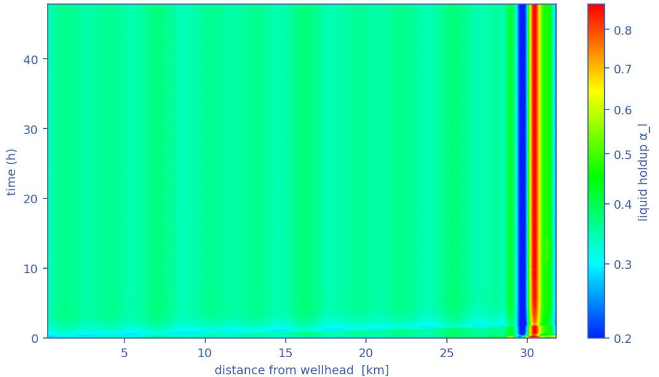
Output — transient liquid-holdup field \alpha_l(x,t)
