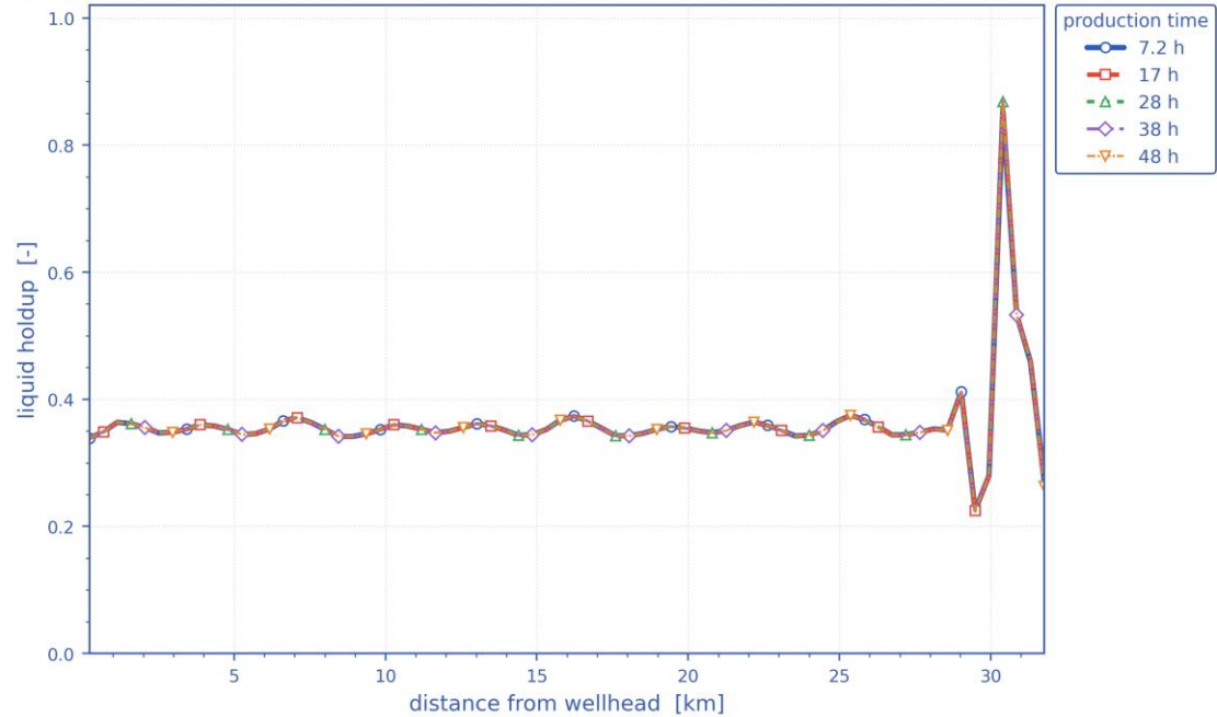
Distribution of liquid holdup along the pipeline after different production durations — engineered fix (insulation + MEG)
