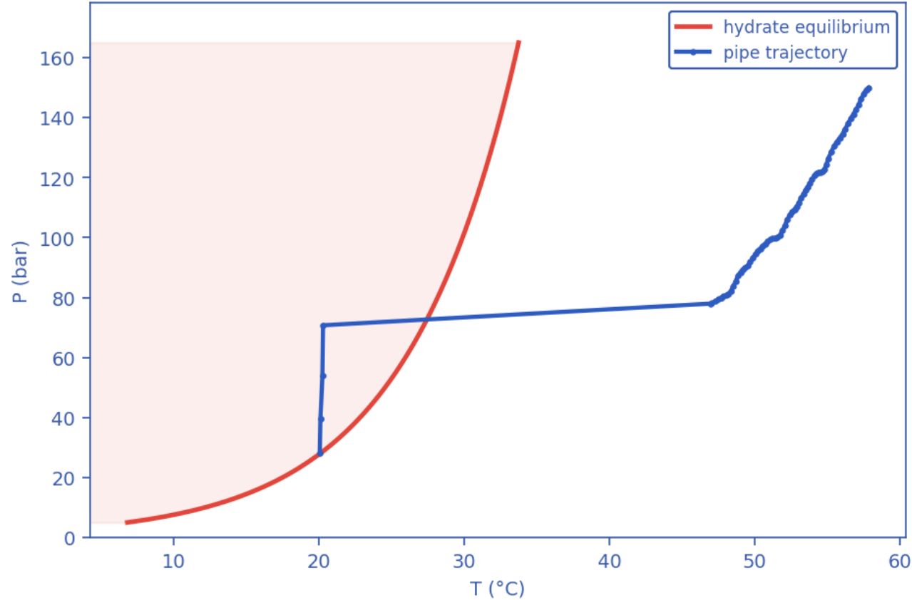
Output C — P-T trajectory vs hydrate envelope
