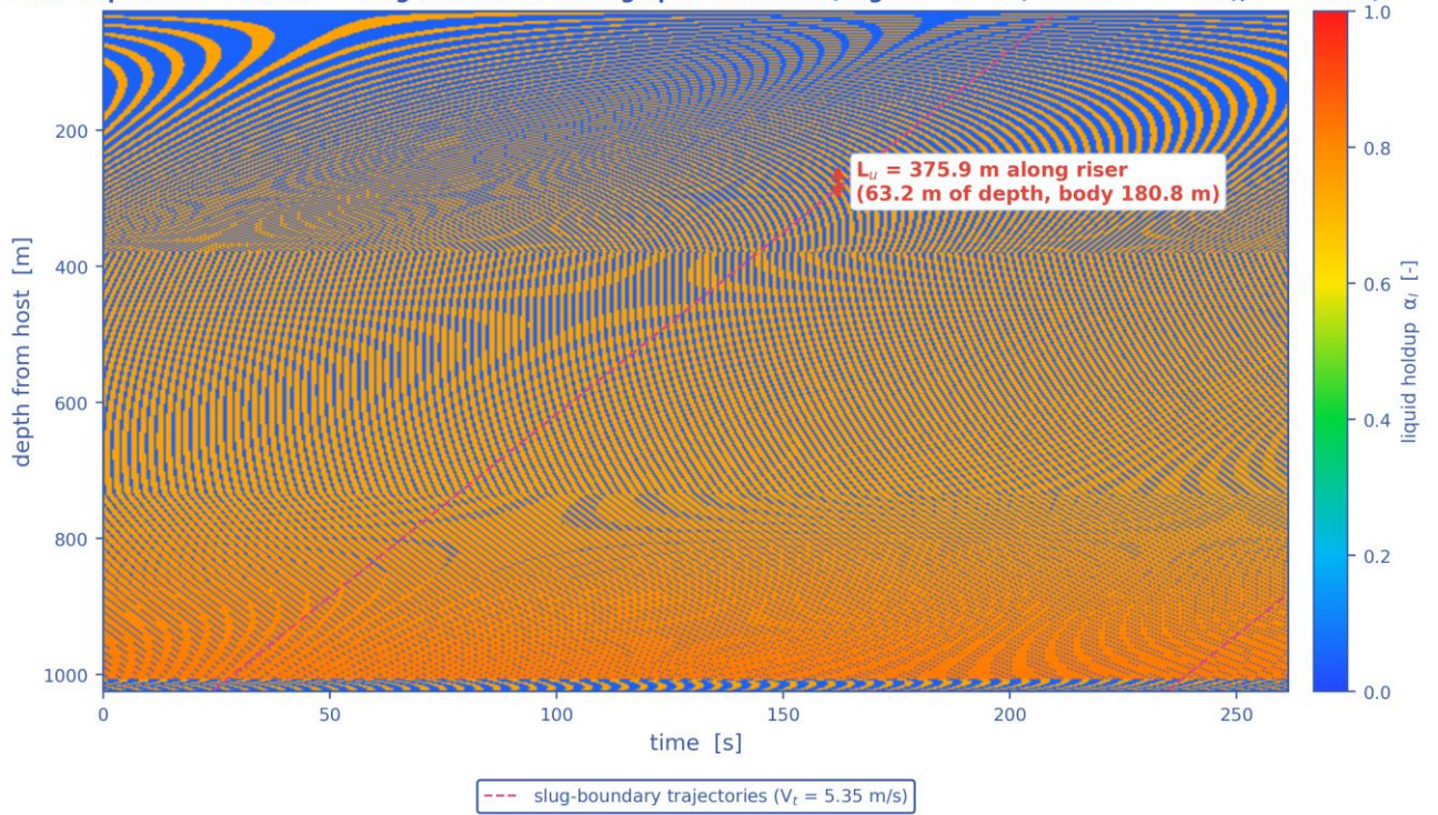
Riser depth-time waterfall — slug boundaries during upward motion (engineered fix (insulation + MEG), t = 47.8 h)
