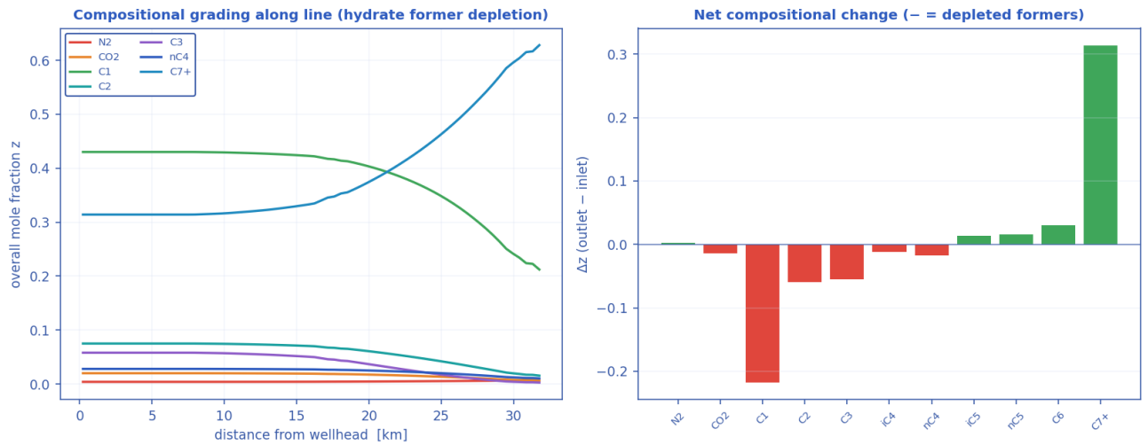
Compositional grading along the route — preferential depletion of the hydrate-forming light ends. [as-operated]
