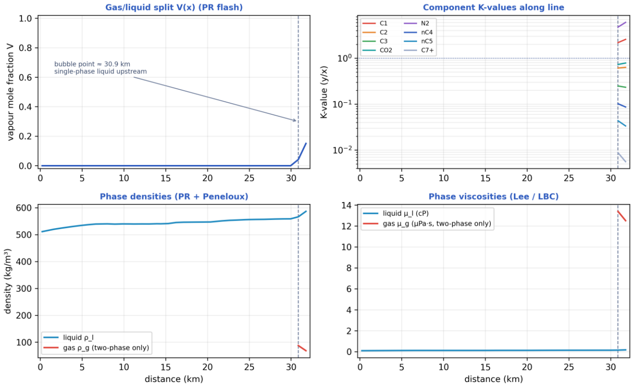
Compositional PVT tracking along the line (Peng–Robinson flash): gas/liquid split, K-values, densities. [as-operated]
