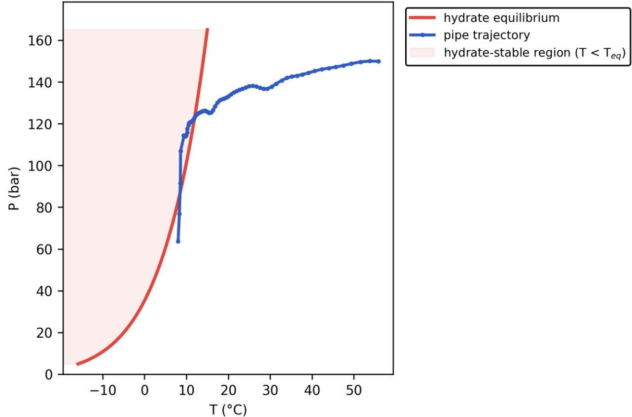
Production P–T trajectory against the hydrate-stability envelope (curve). [as-operated]
