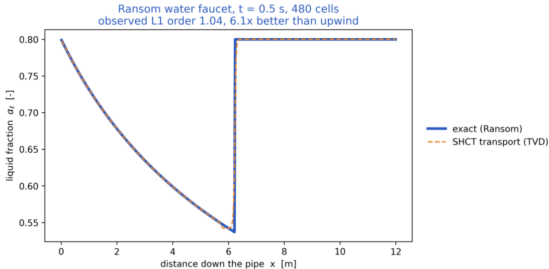
Ransom water-faucet benchmark: the solver's holdup transport against the exact solution. L1 error converges at first order across the front, where L-infinity does not converge at all and L2 converges only at O(h^{1/2}) .
