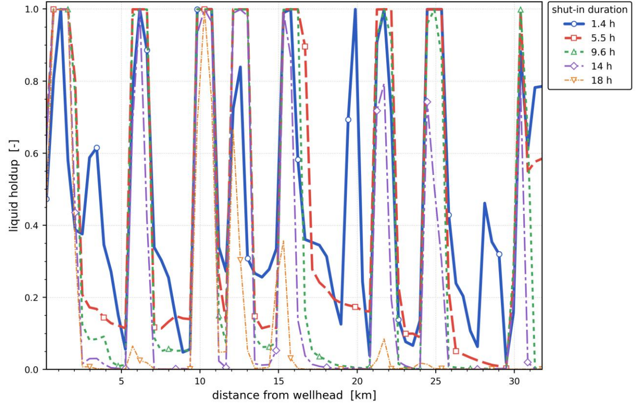
Distribution of liquid holdup along the pipeline after successive elapsed durations (shut-in duration for the shut-in scenario, production time otherwise) — one curve per duration. [shut-in]
