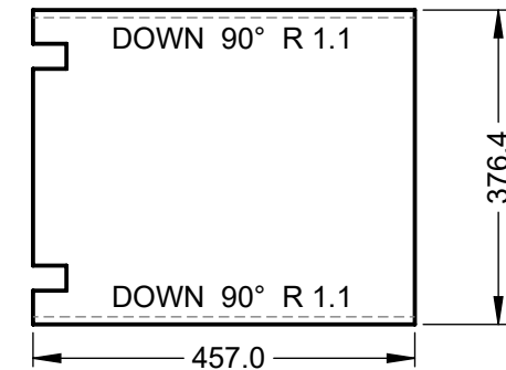
(FLAT PATTERN)
