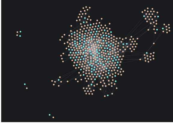
Fig. 4. Graph database.
