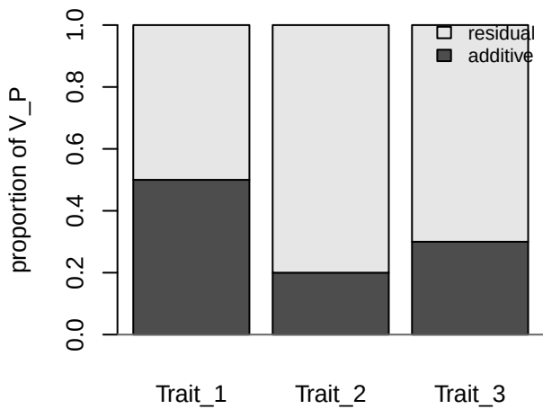
Variance partition
