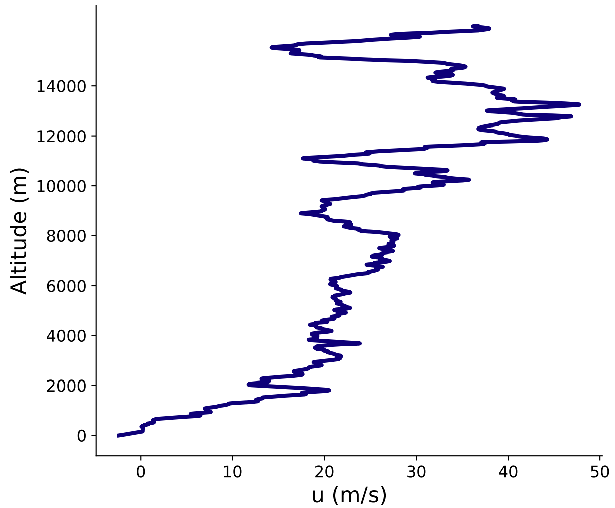
Zonal Wind
