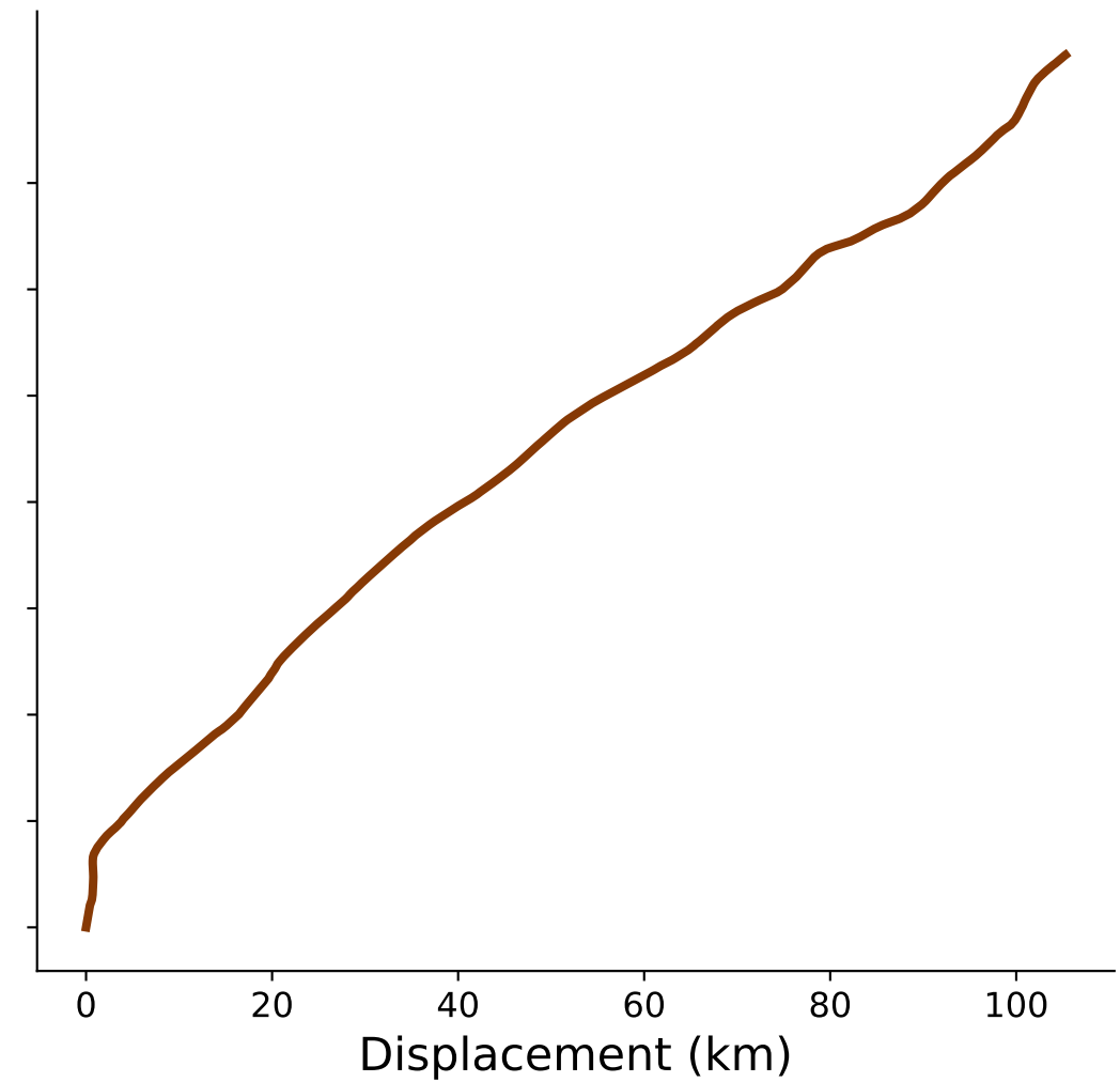
Horizontal Drift
