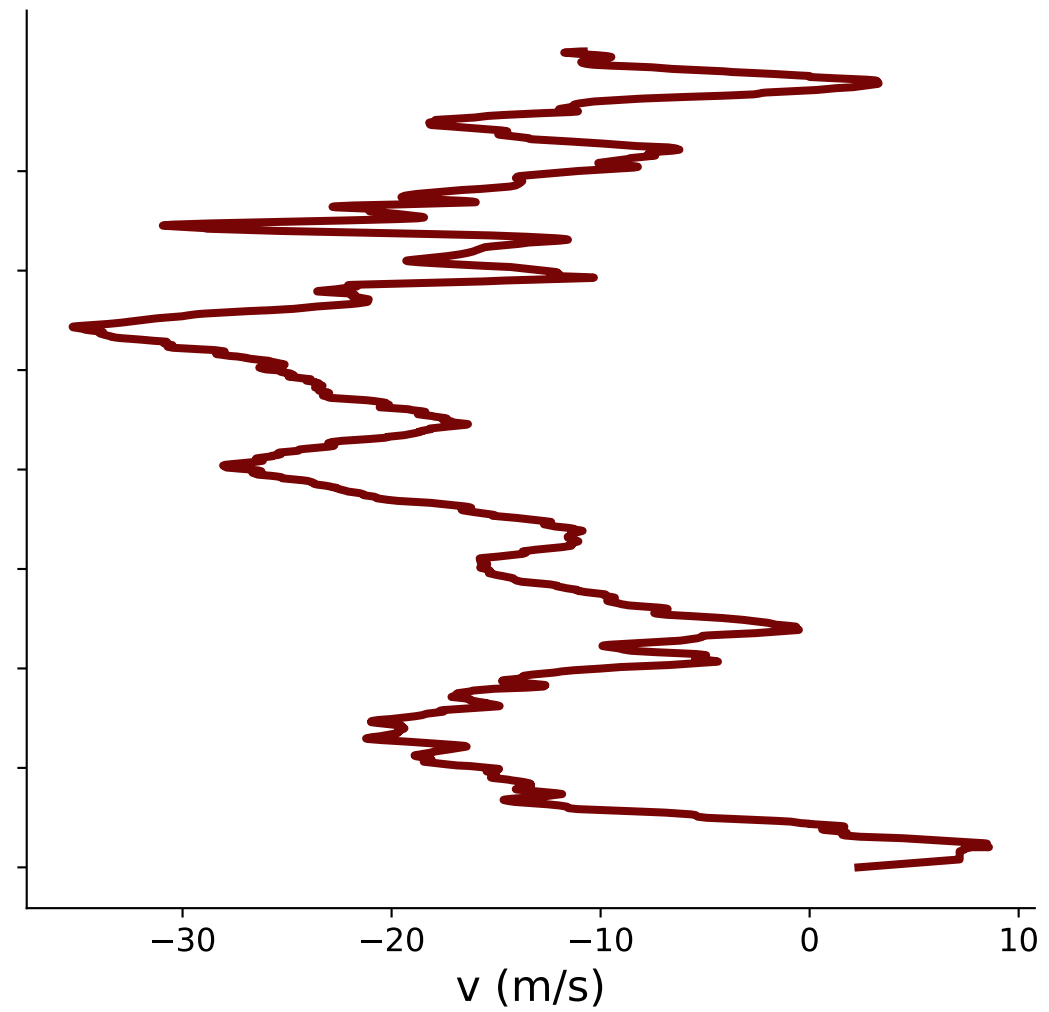
Meridional Wind
