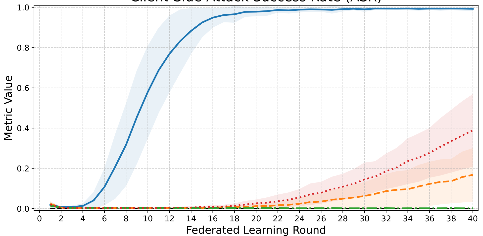
Client-Side Attack Success Rate (ASR)
