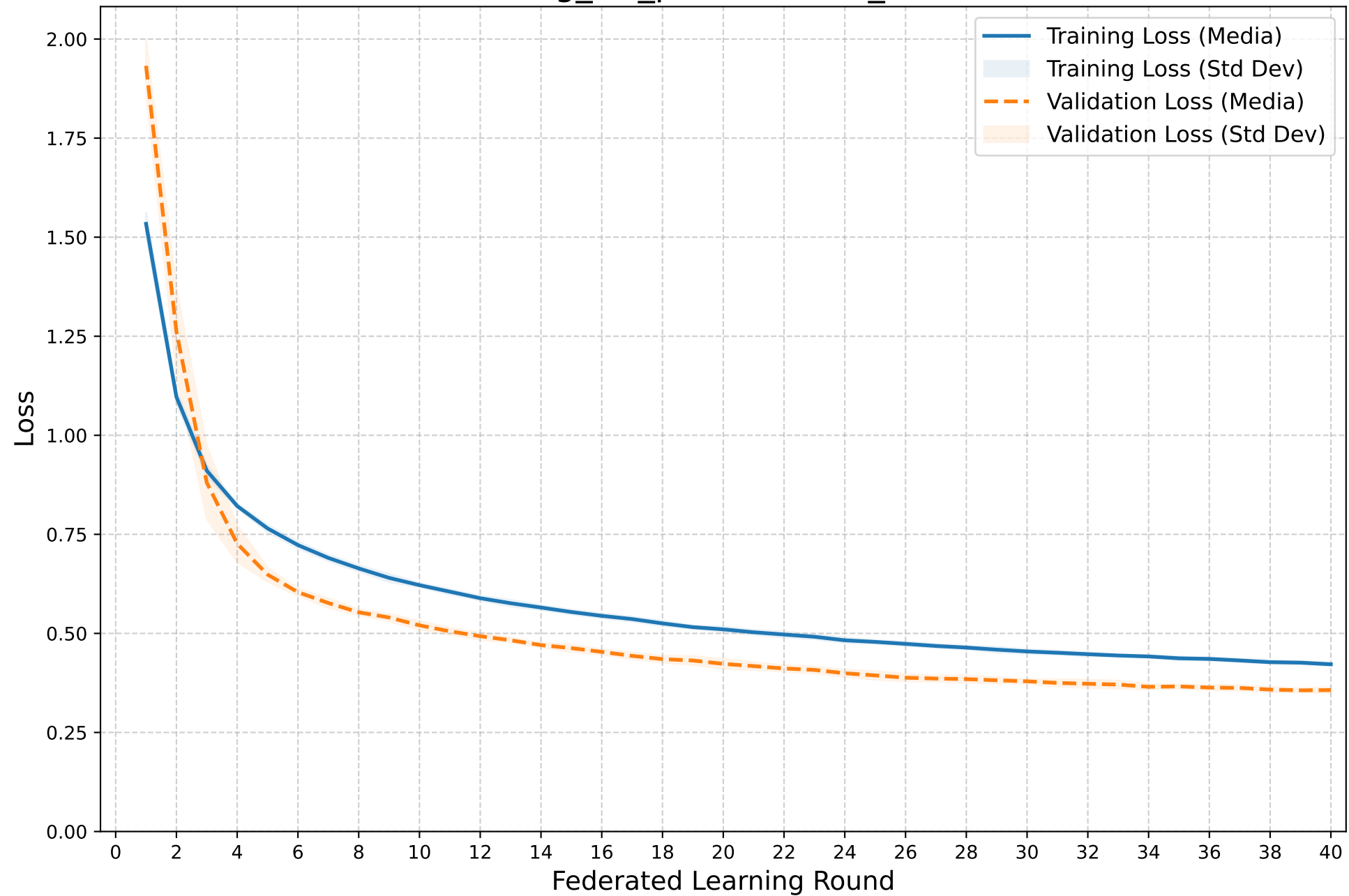
Training vs Validation Loss FedAvg_IID_personalized_frac08
