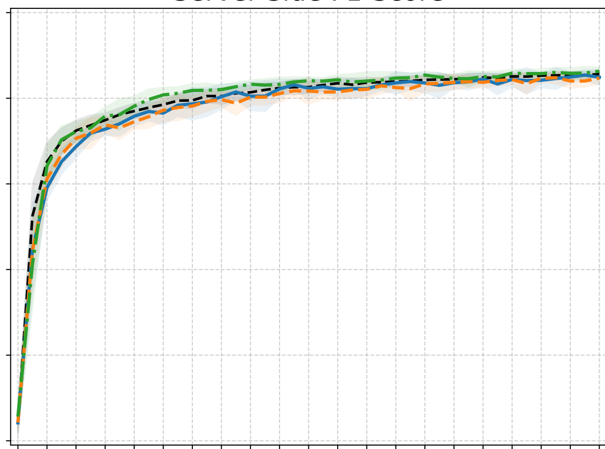
Server-Side F1-Score
