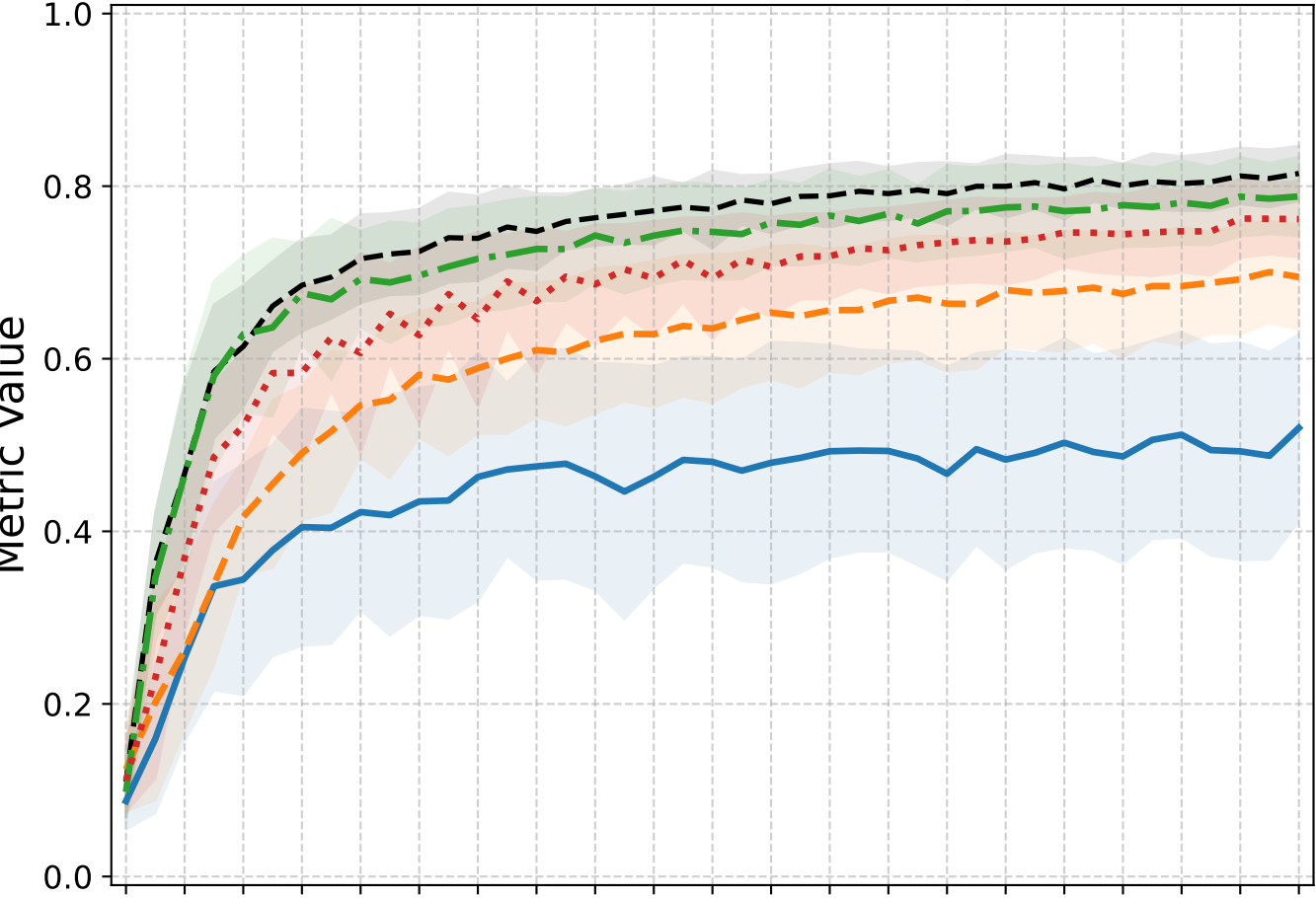
Server-Side Accuracy
