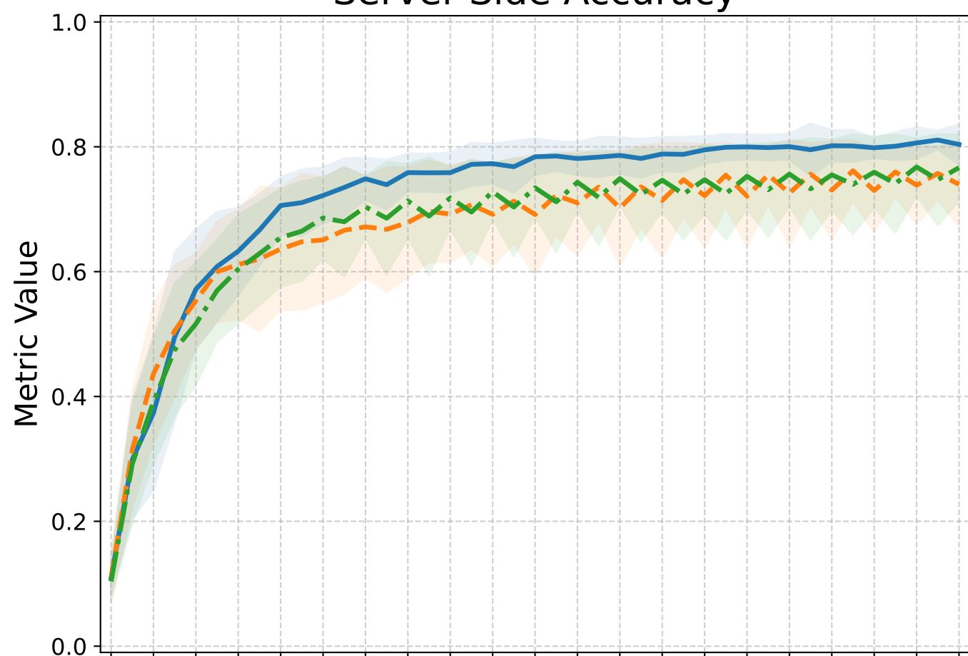
Server-Side Accuracy
