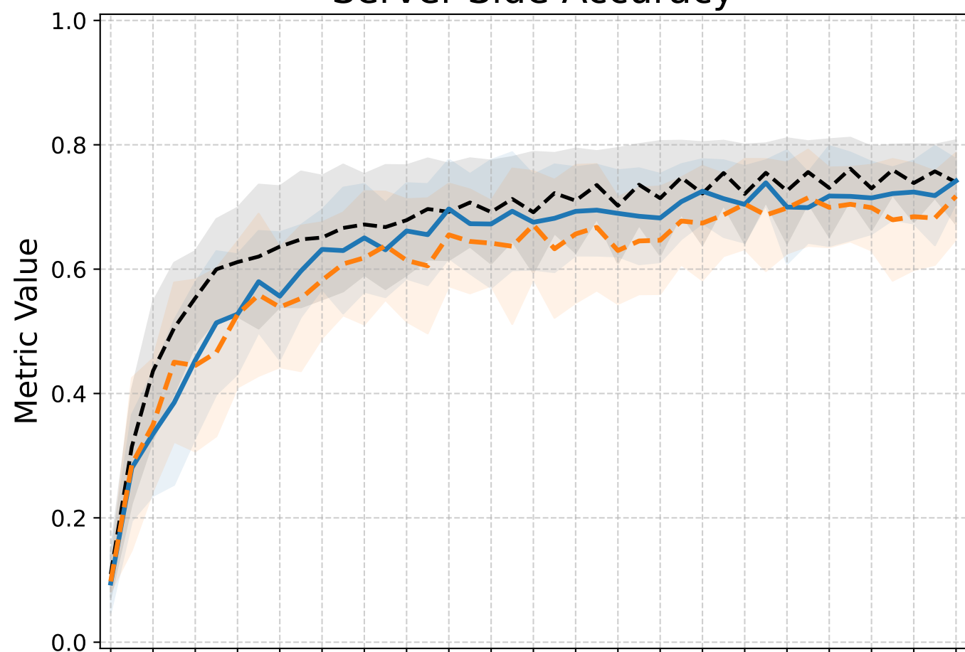
Server-Side Accuracy
