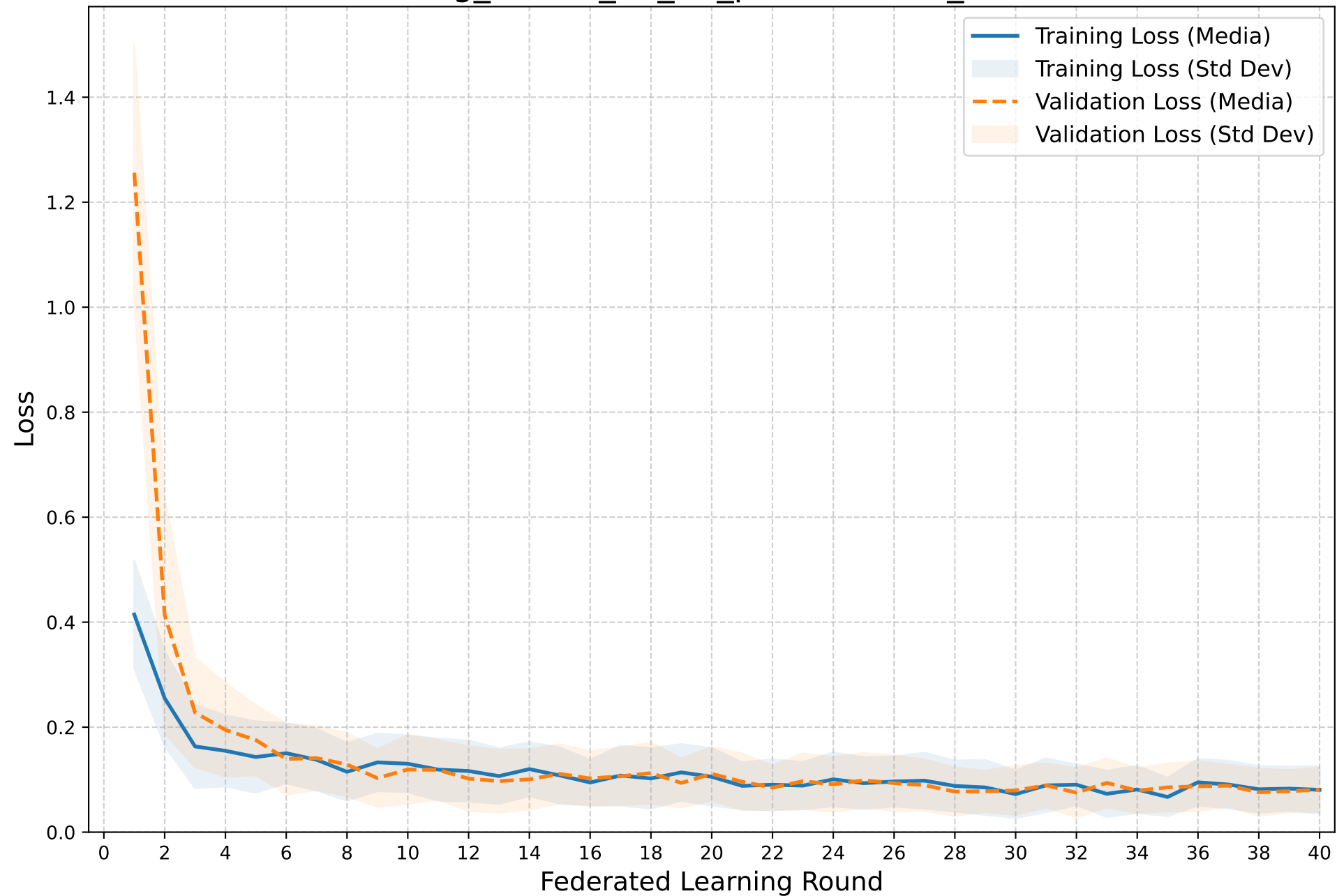
Training vs Validation Loss FedAvg_nonIID_a0_03_personalized_frac08
