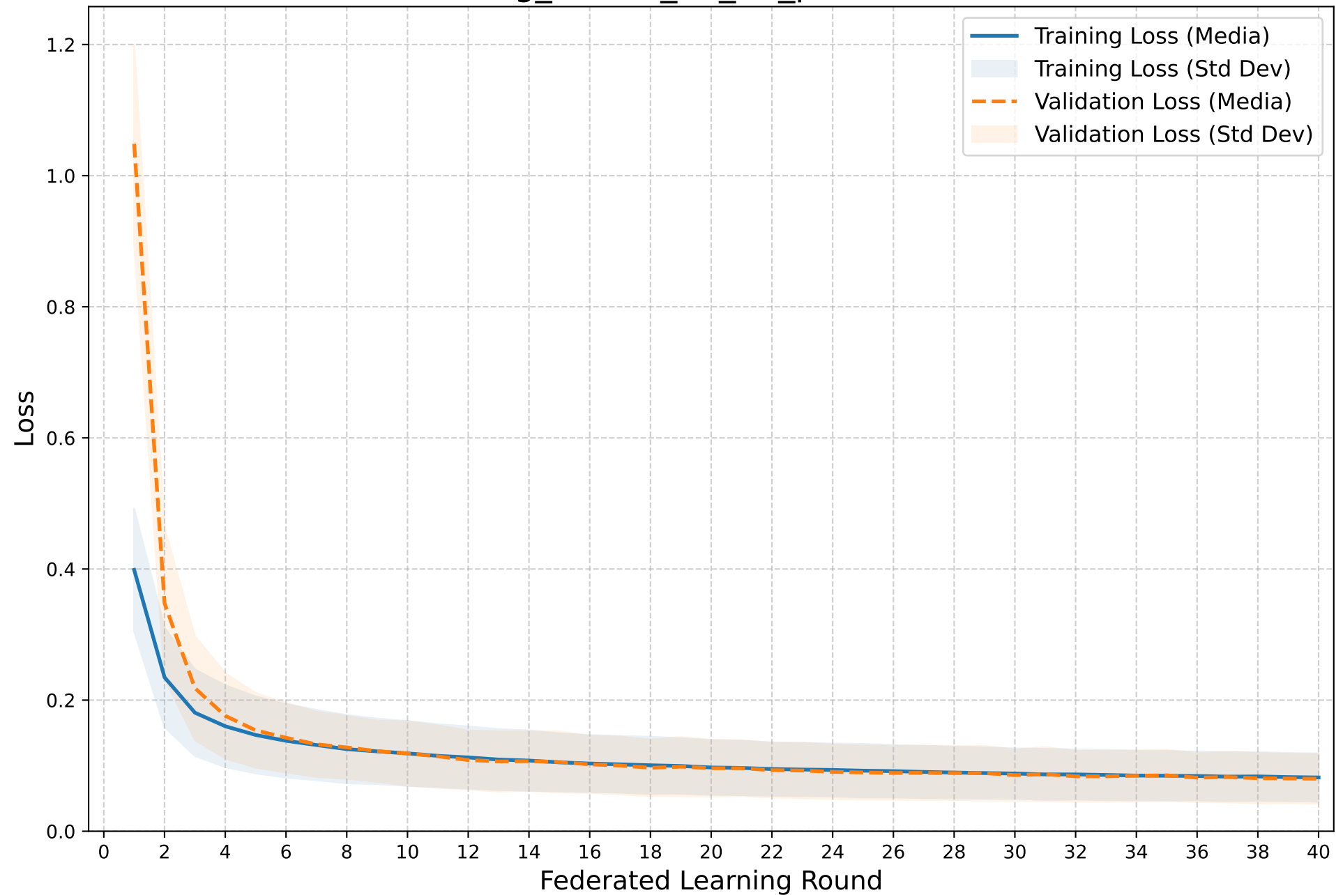
Training vs Validation Loss FedAvg_nonIID_a0_03_personalized
