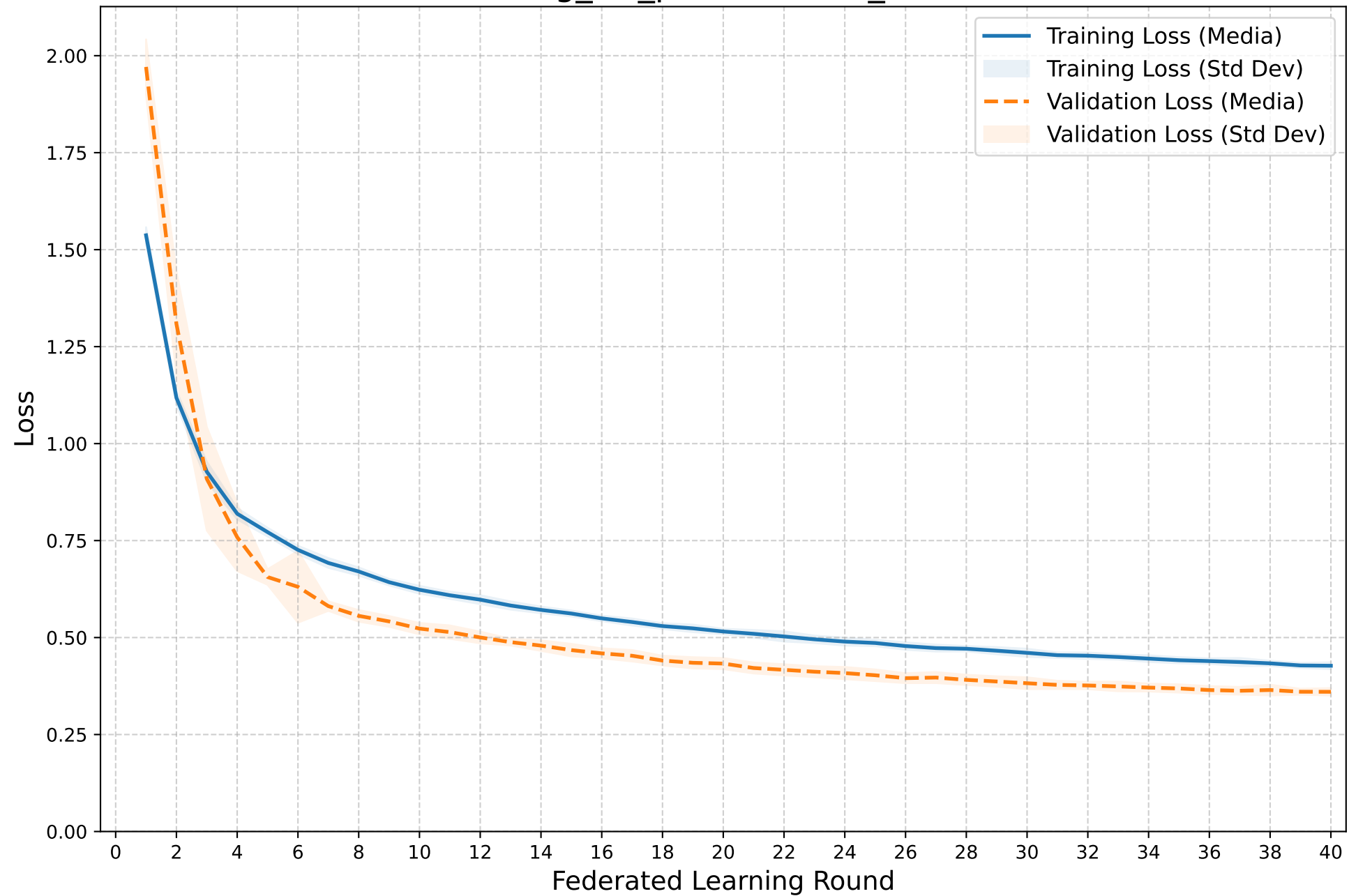
Training vs Validation Loss FedAvg_IID_personalized_frac07
