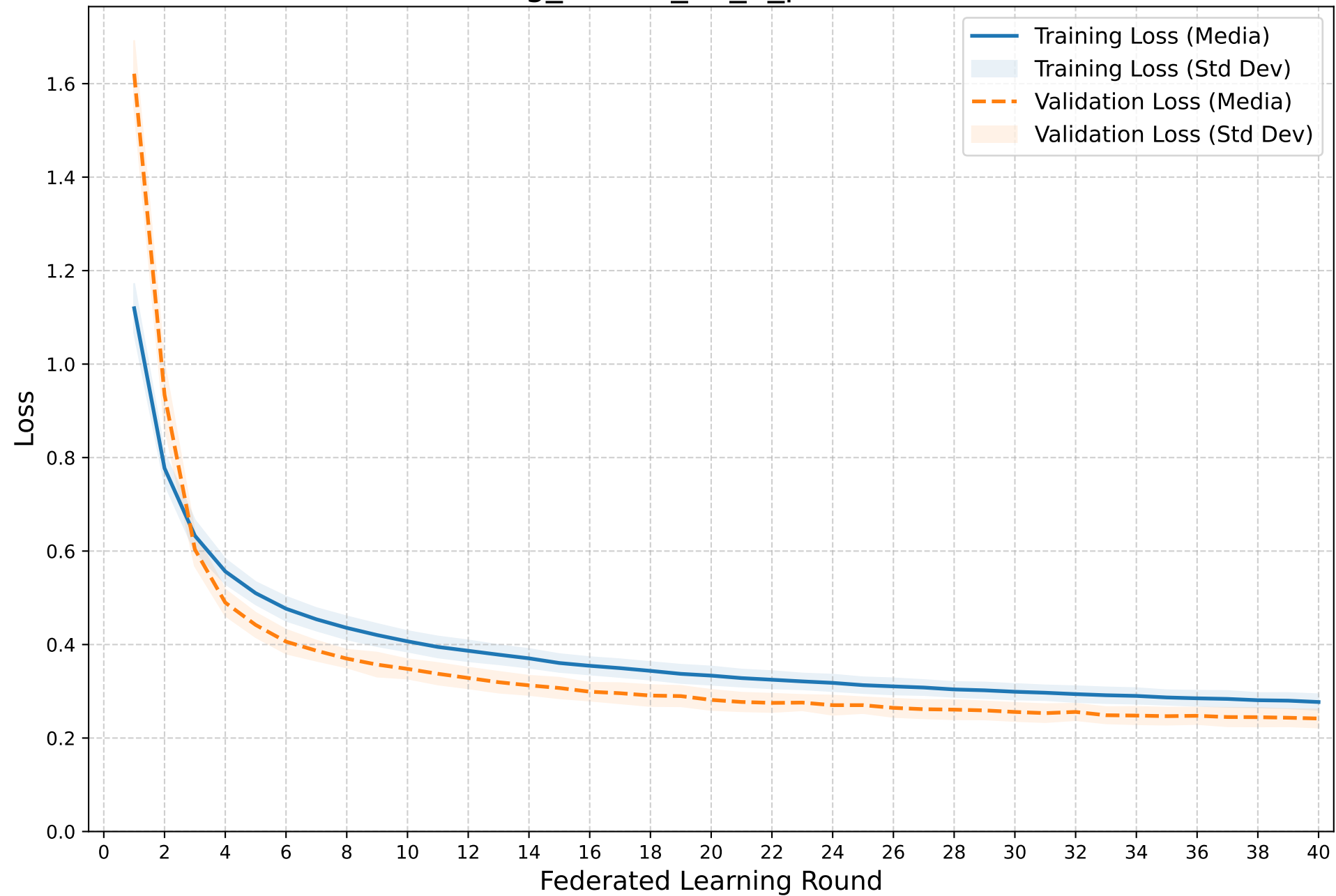
Training vs Validation Loss FedAvg_nonIID_a0_5_personalized
