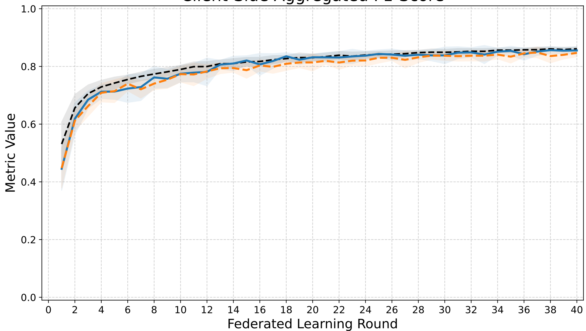
Client-Side Aggregated F1-Score
