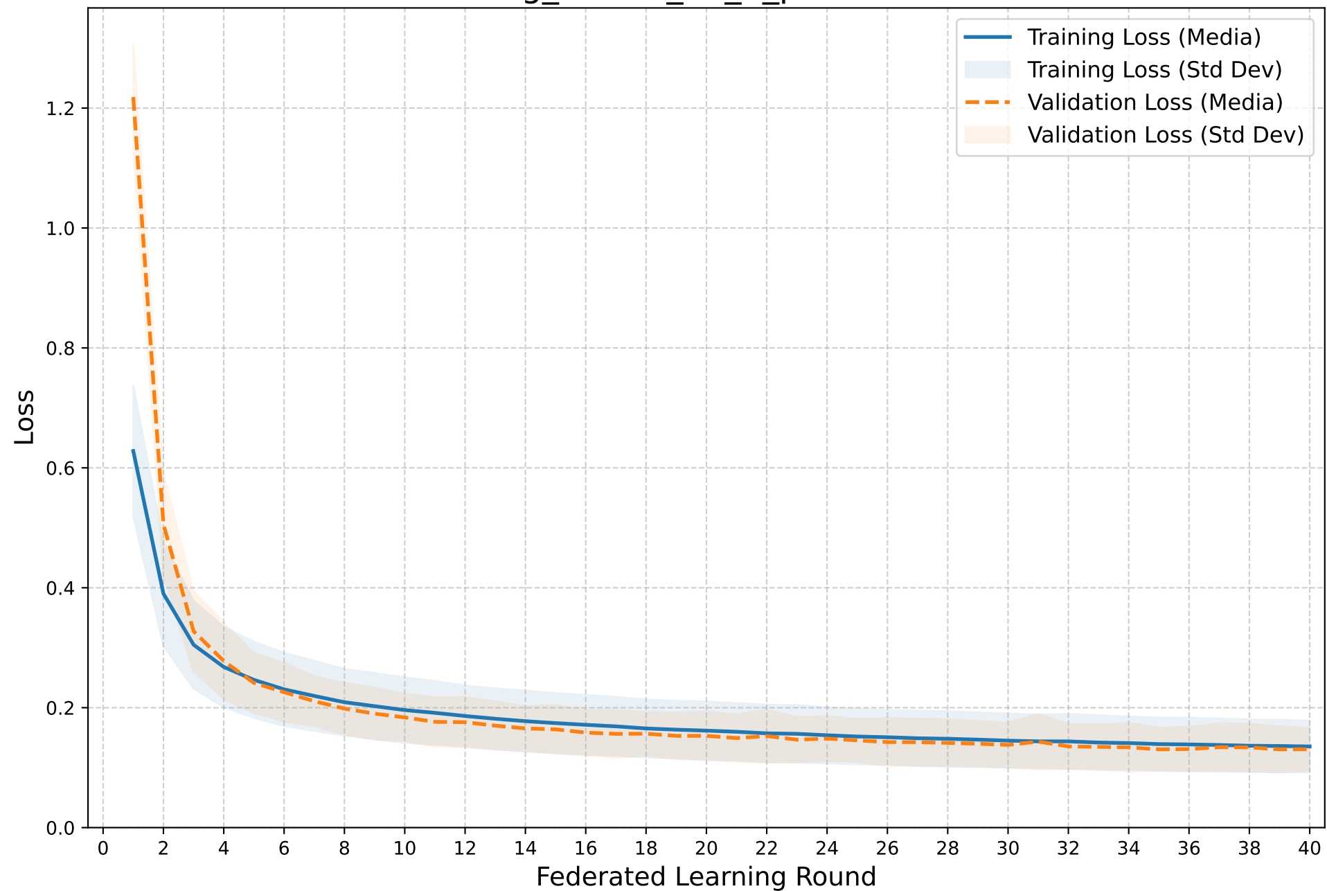
Training vs Validation Loss FedAvg_nonIID_a0_1_personalized
