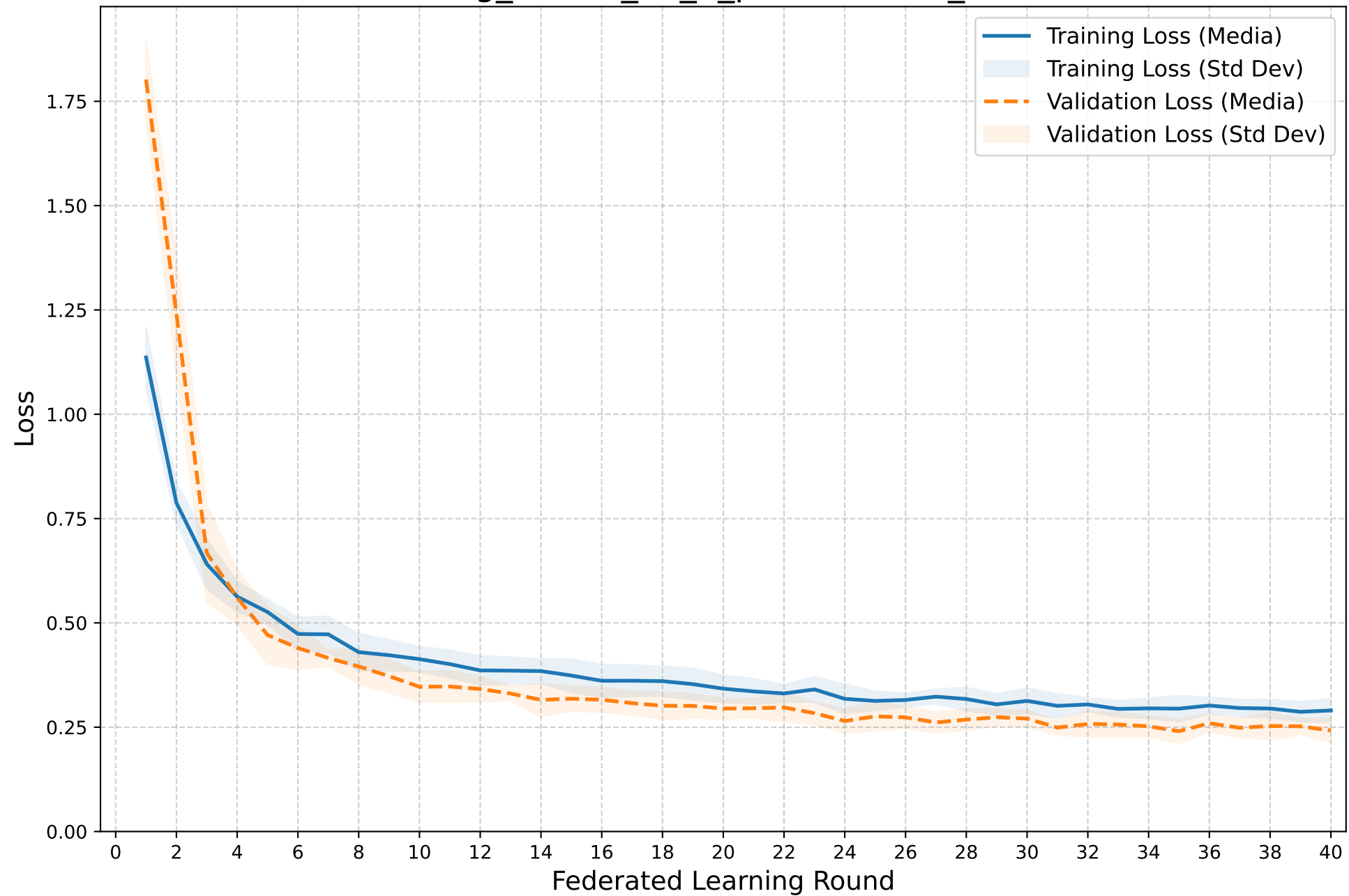
Training vs Validation Loss FedAvg_nonIID_a0_5_personalized_frac07
