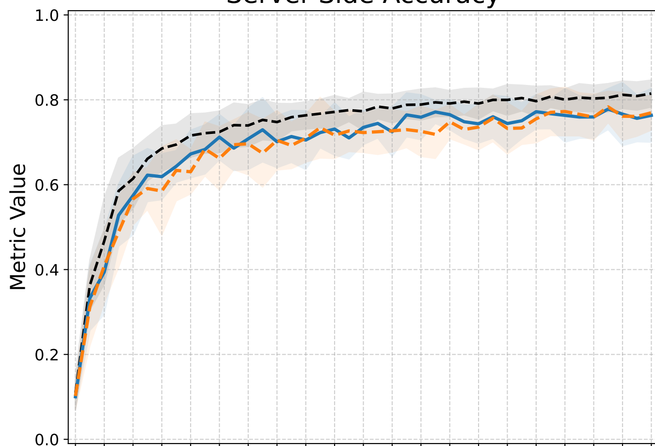
Server-Side Accuracy
