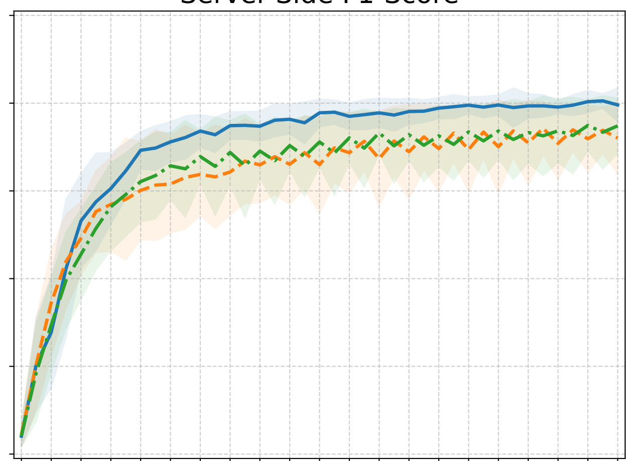
Server-Side F1-Score
