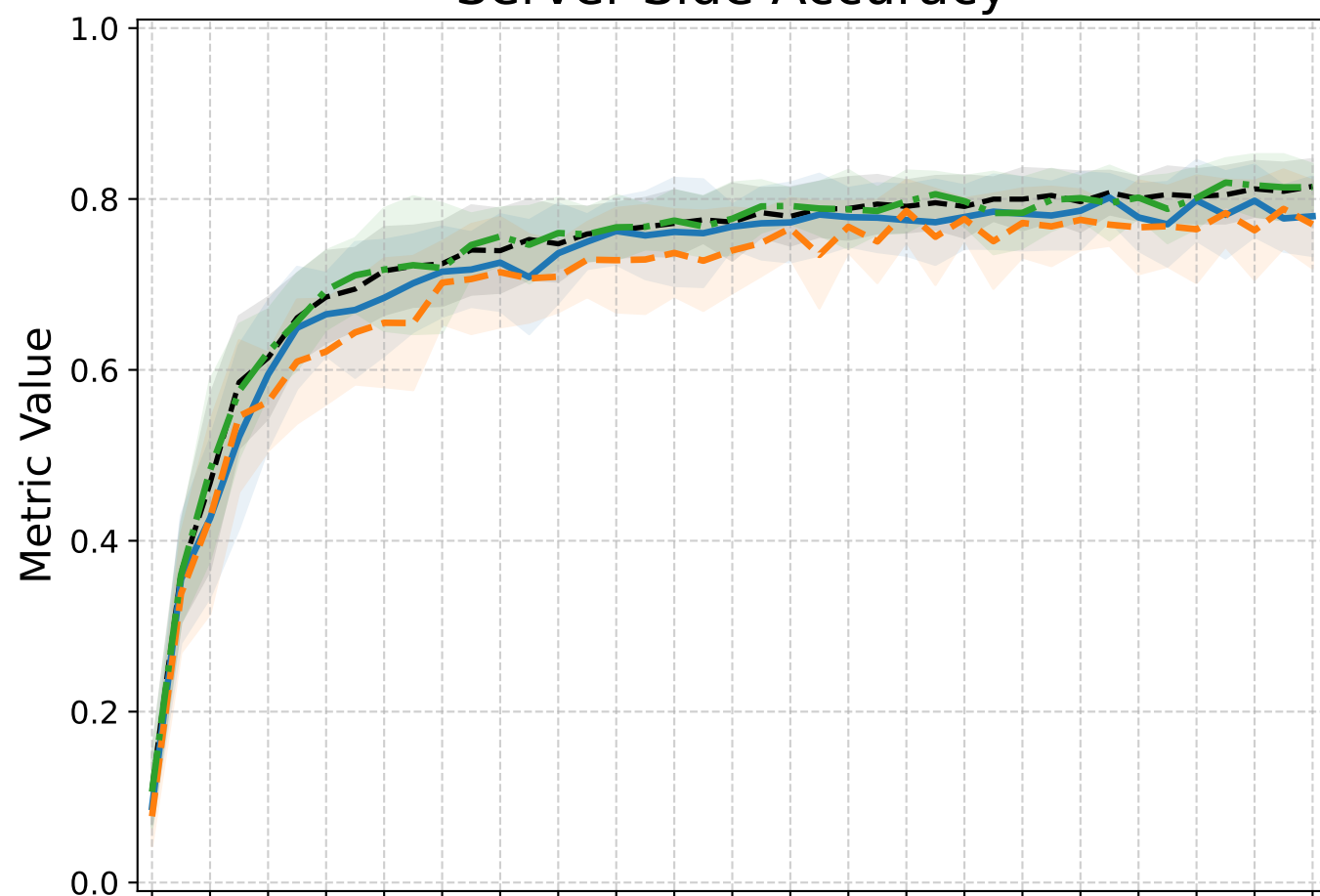
Server-Side Accuracy
