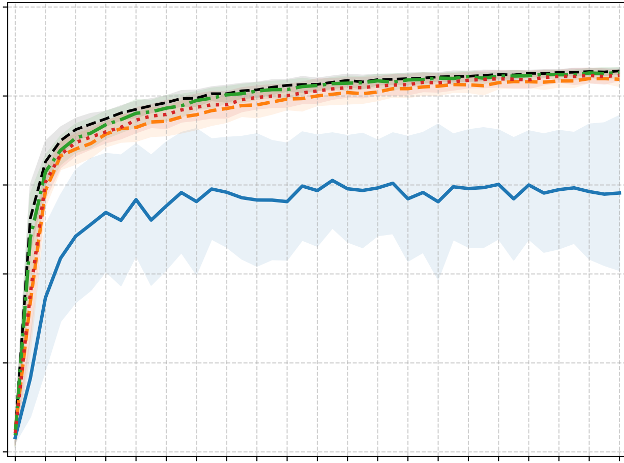
Server-Side F1-Score
