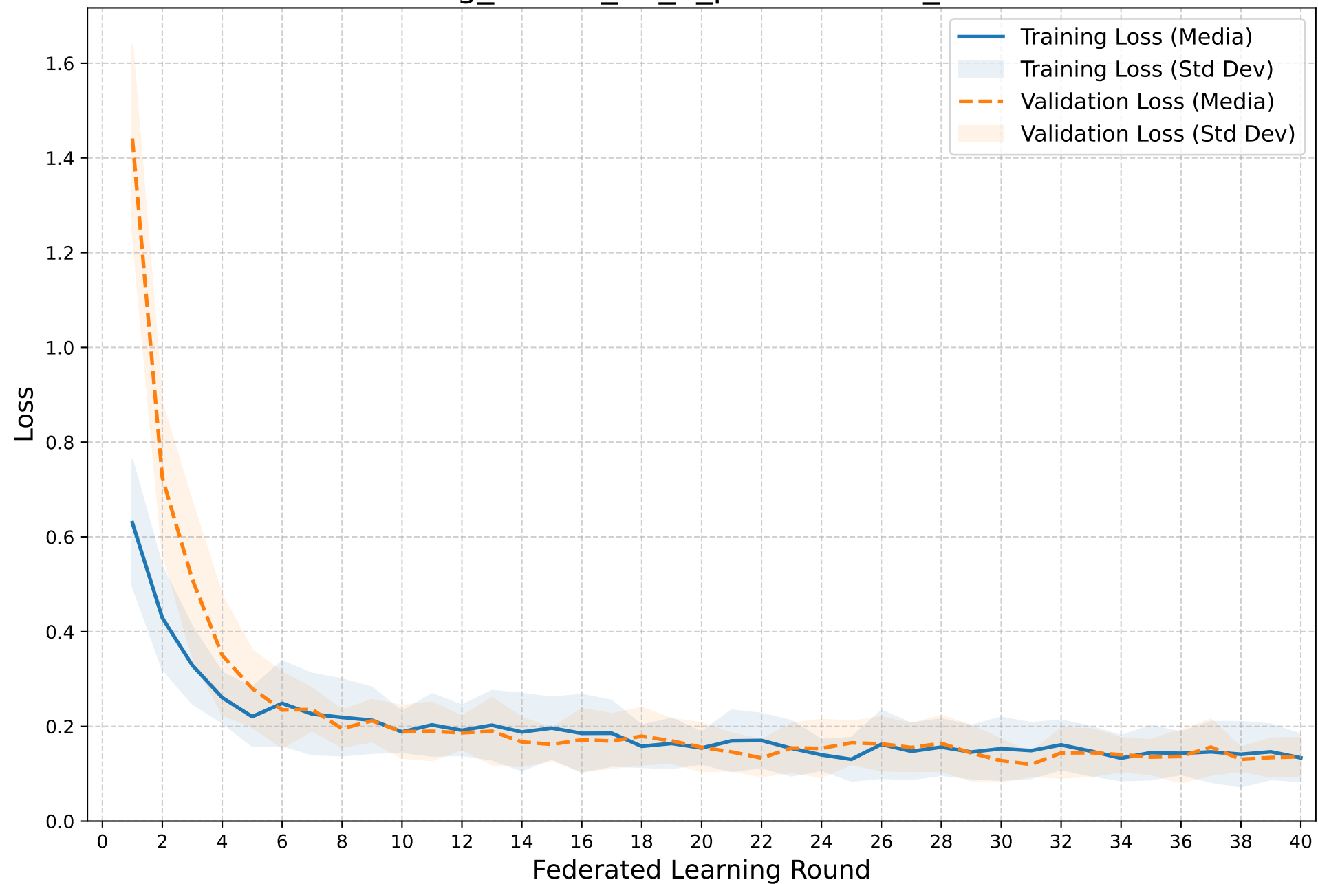
Training vs Validation Loss FedAvg_nonIID_a0_1_personalized_frac07
