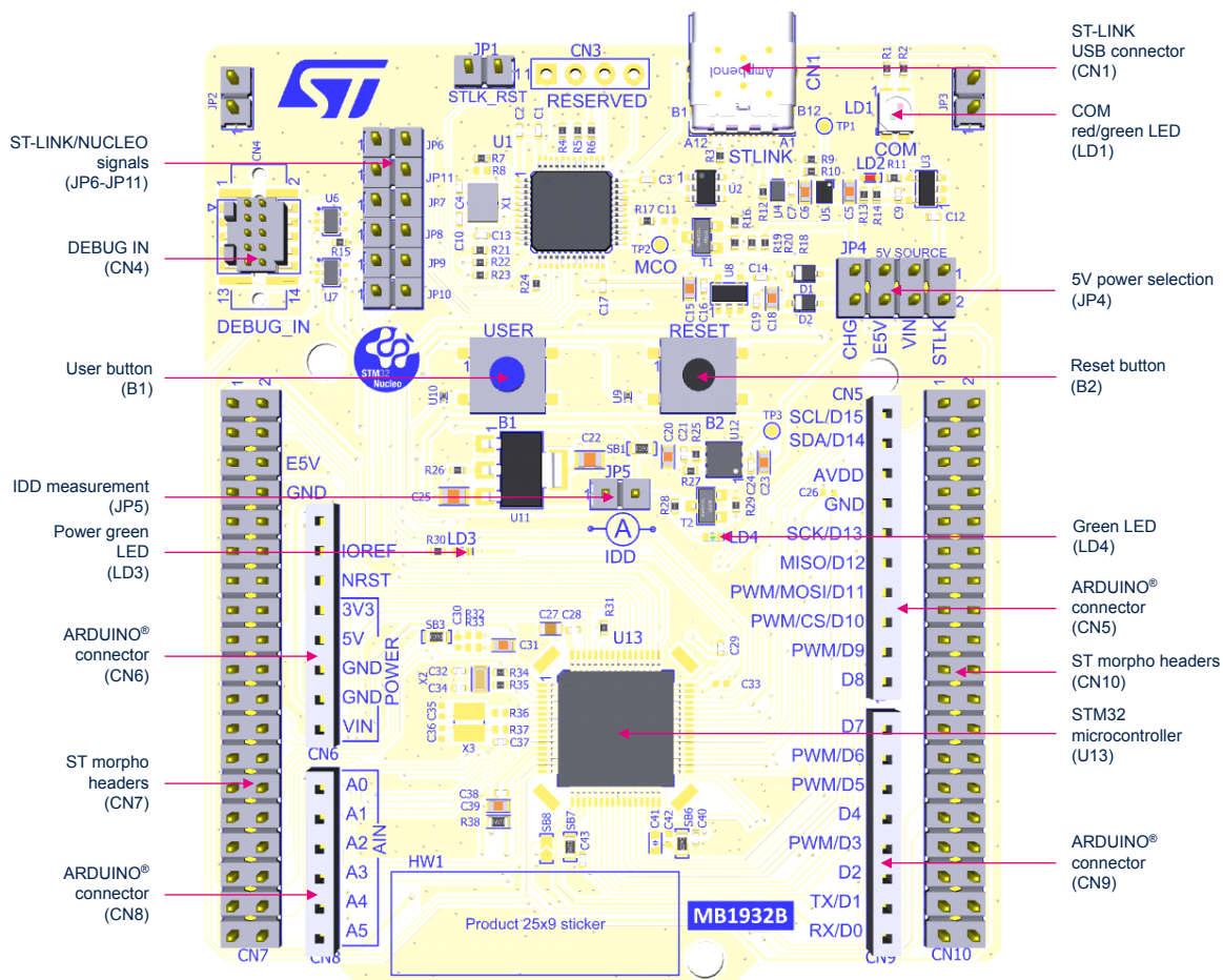
Figure 3. Top layout
