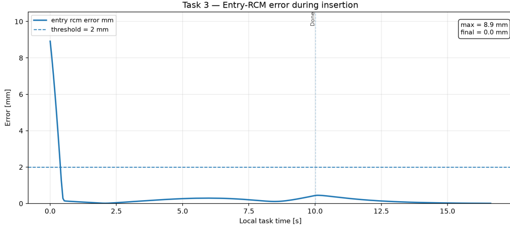
Figure 4: Task 3 entry-RCM error during insertion. The 8.9 mm raw peak is a phase-entry transient; after the 1 s settling interval the maximum is 0.423 mm (2 mm threshold).
