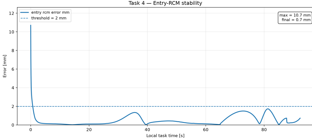
Figure 9: Task 4 entry-RCM error. Raw maximum: 10.701 mm; settled validation maximum: 1.727 mm against 2 mm.
