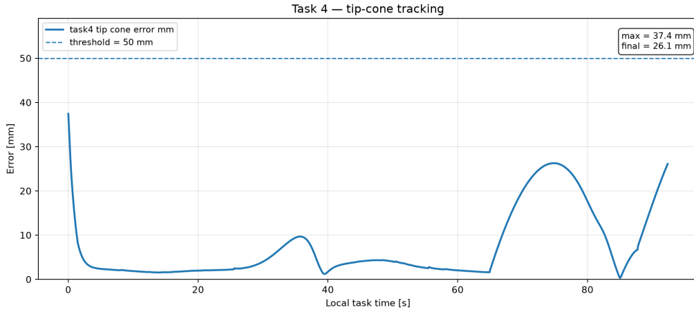
Figure 10: Task 4 tip-cone error. Raw maximum: 37.427 mm; settled validation maximum: 26.260 mm against 50 mm.
