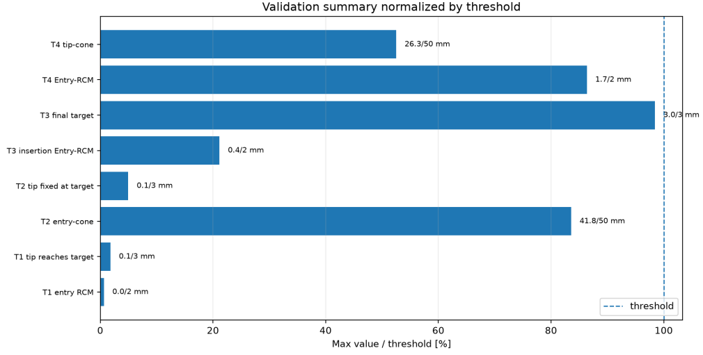
Figure 2: Validation summary normalized by threshold. Results obtained from the logged experimental run.
