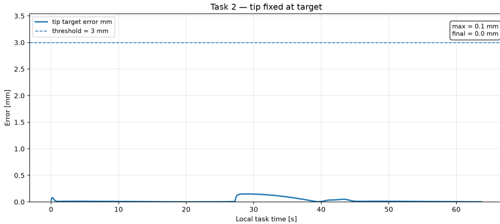
Figure 8: Task 2 primary tip-target error: 0.149 mm maximum against the 3 mm threshold.
