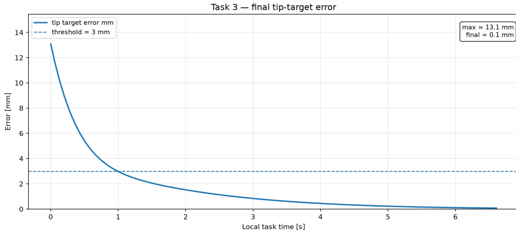
Figure 5: Task 3 tip-to-target error in the Done phase. The settled maximum is 2.953 mm and the final recorded error is 0.074 mm (3 mm threshold).
