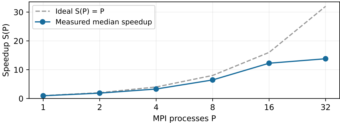
Square: 16384 x 16384, CAPRI final campaign
