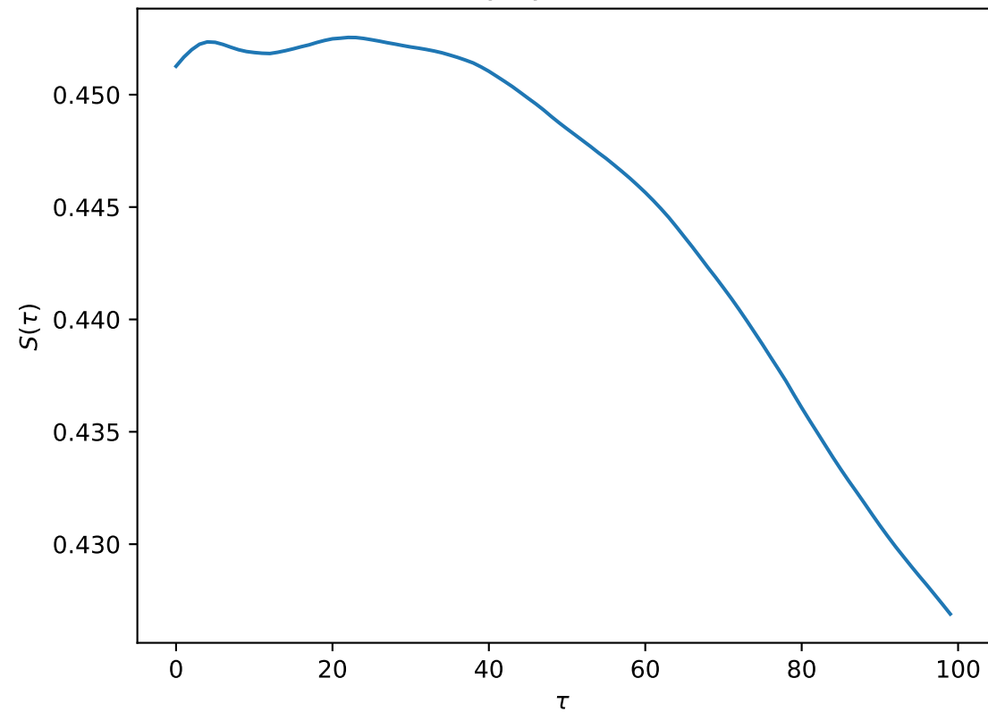
Generally-Synchronized JRP
