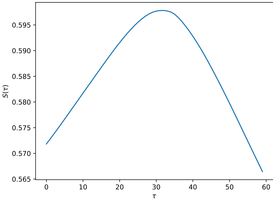
Phase-Synchronized JRP
