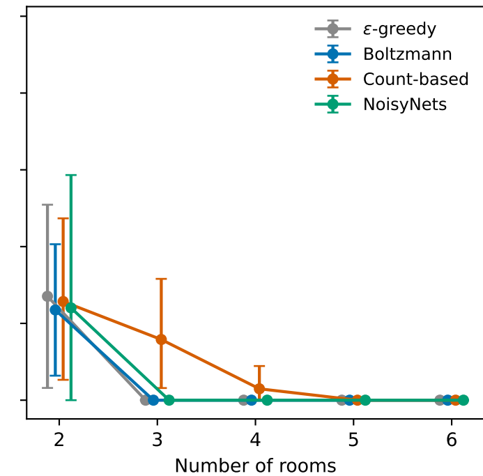
MultiRoom
