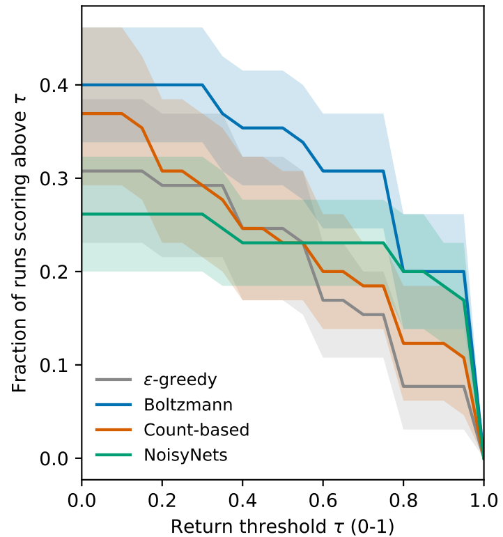
Performance profile, all instances
