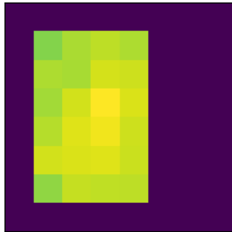
Count-based
