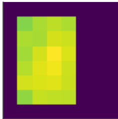
Count-based
