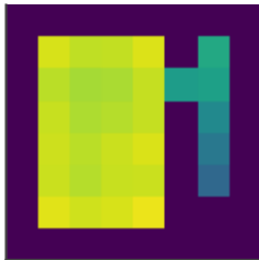
Boltzmann
