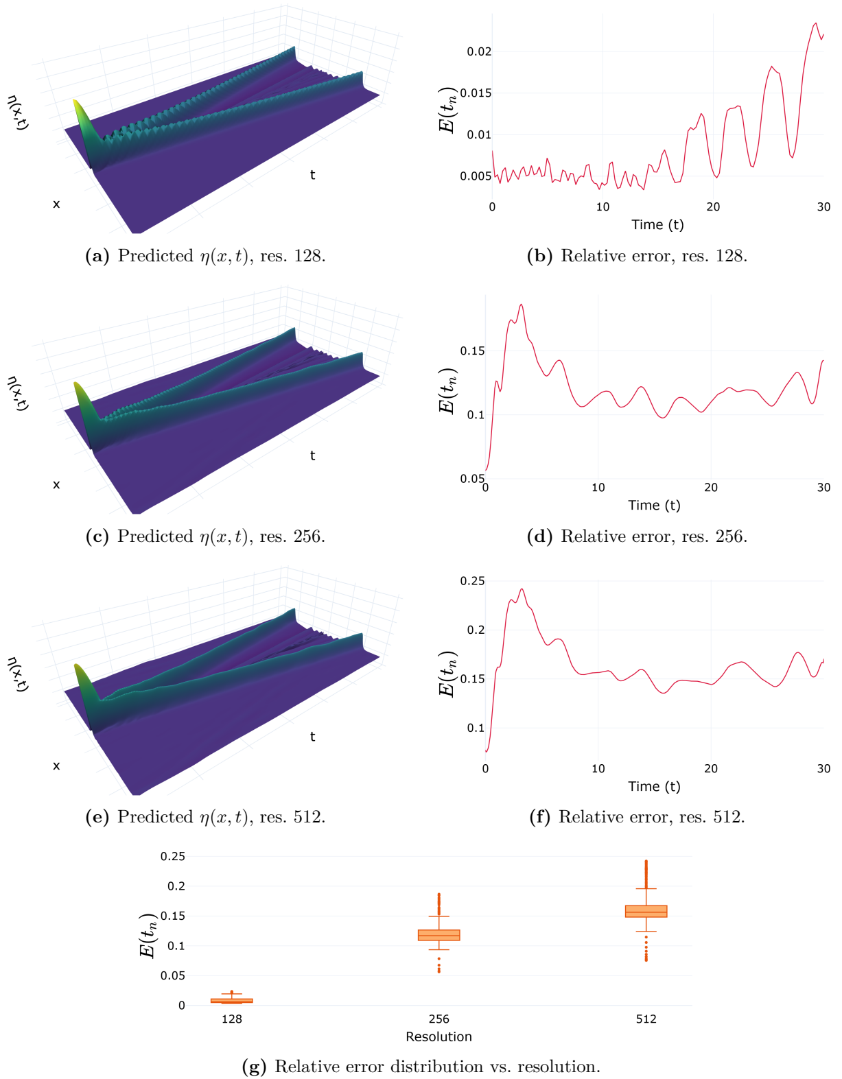
Figure 4.6 – Plain FNO queried zero-shot at resolutions 128, 256 and 512 at \alpha = \beta = 3,21 . Predicted \eta(x, t) and time-resolved relative error E(t_n) of (3.8) at each resolution.
