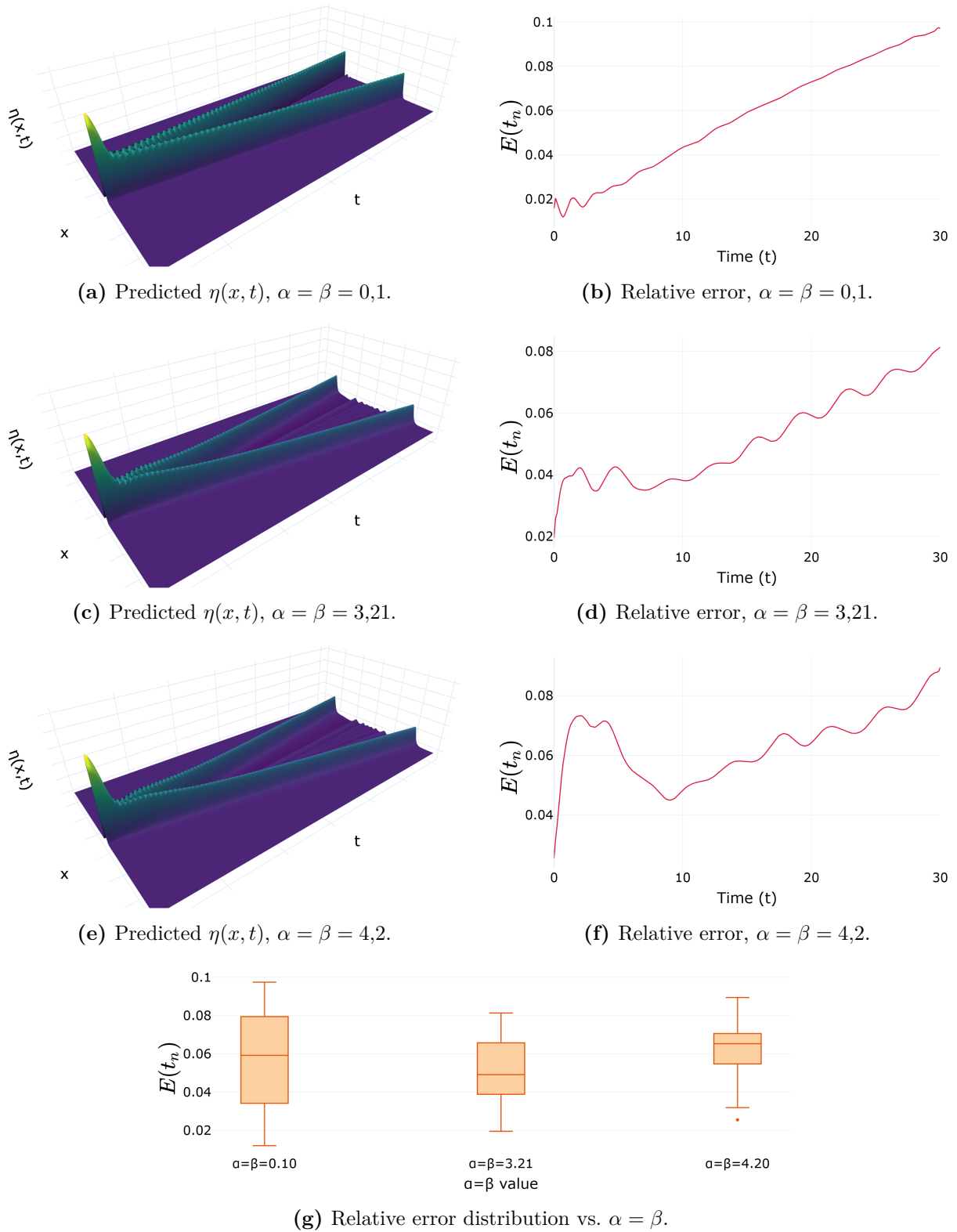
Figure 4.4 – PINO (data and physics) across the same nonlinearity axis and resolution. Left: predicted \eta(x, t) . Right: time-resolved relative error E(t_n) of (3.8).
