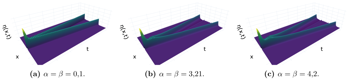
Figure 4.1 – Reference solution \eta(x, t) of (4.1) computed by the pseudospectral solver at resolution 256.
