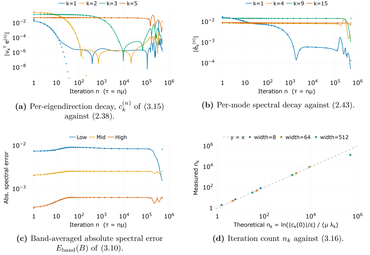
Figure 4.15 – Spectral bias predictions measured in the minimal experiment of Section 3.5, the Spectral Bias MLP fitting \eta(x, 15) at \alpha = \beta = 3, 21 by full-batch gradient descent at the per-width step (3.14), run for 500,000 iterations. Panels (a)–(c) are the widest network, N_{\text{MLP}} = 512 ; panel (d) collects all three widths. Lines are measured, open markers are the initial-kernel prediction.
