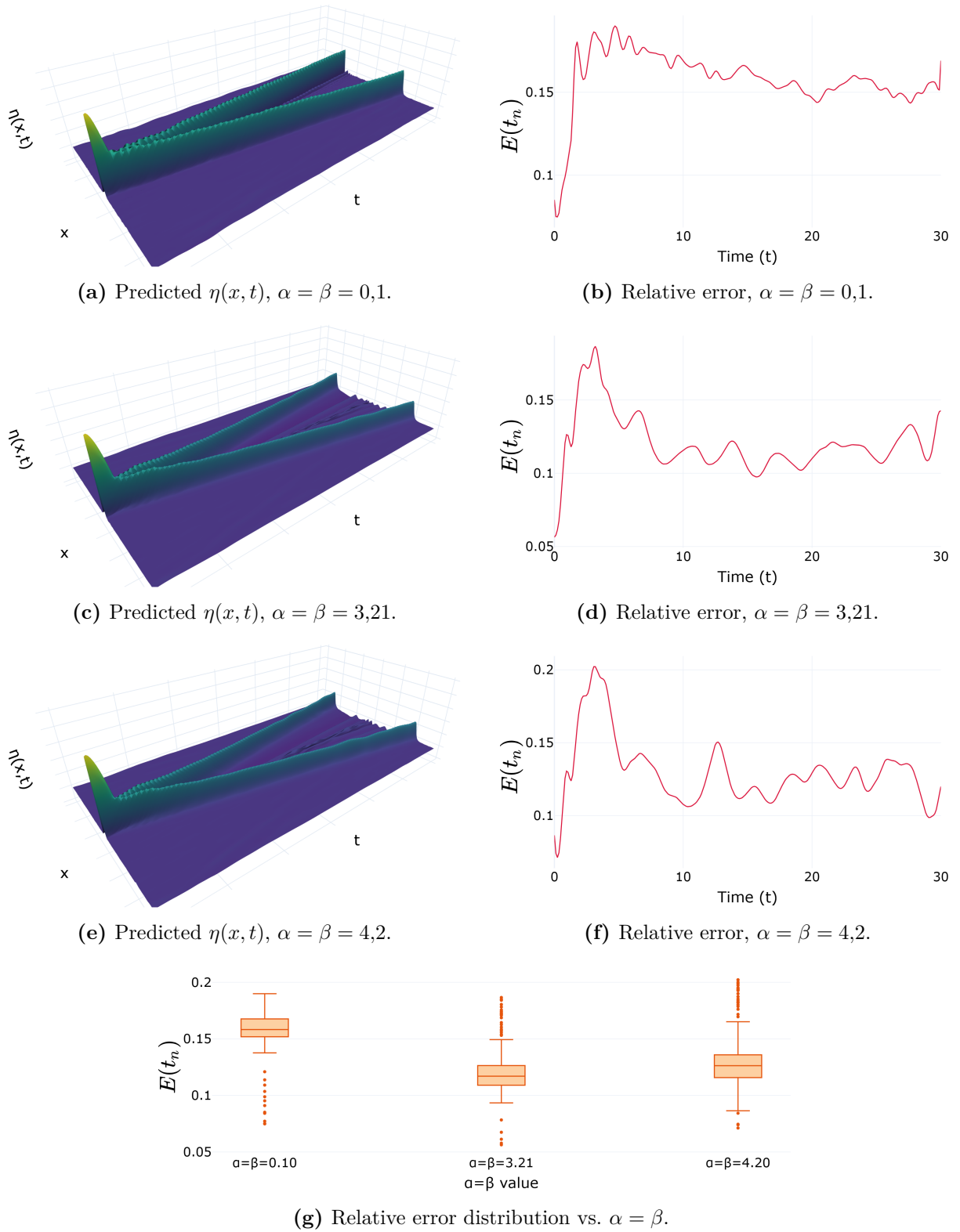
Figure 4.3 – FNO (pure data) across the nonlinearity axis ( \alpha = \beta \in \{0,1; 3,21; 4,2\} ), evaluated at resolution 256. Left: predicted \eta(x, t) . Right: time-resolved relative error E(t_n) of (3.8).
