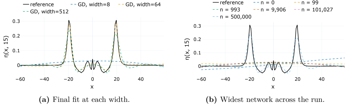
Figure 4.16 – The Spectral Bias MLPs against the reference profile \eta(x, 15) at \alpha = \beta = 3, 21 . Panel (a) shows the final fit at each width; panel (b) follows the widest network across logarithmically spaced checkpoints.
