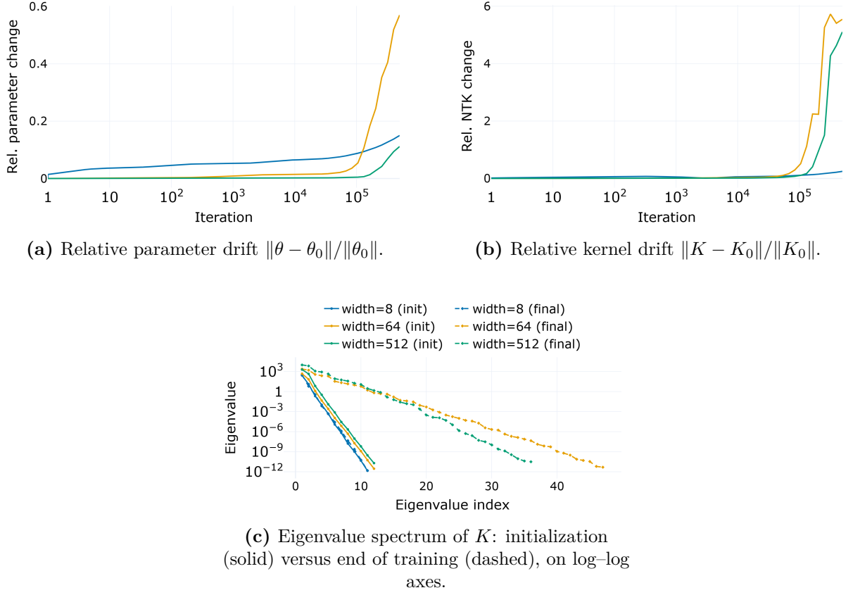
Figure 4.17 – Neural Tangent Kernel diagnostic of Section 3.5.2 for the minimal experiment at \alpha = \beta = 3,21 , logged along the same gradient-descent runs as Figure 4.15, for widths 8, 64 and 512. This figure was made inspired by Wang, Yu, et al. (2022) and Jacot et al. (2018).
