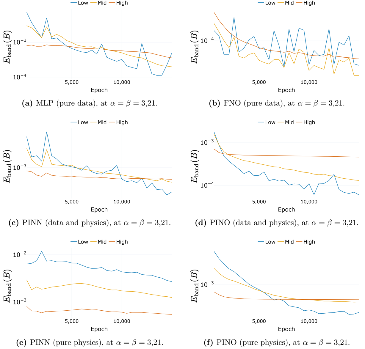
Figure 4.18 – Band-averaged absolute spectral error E_{\text{band}}(B) of (3.10) during training, every method tracked at the common parameter \alpha = \beta = 3,21 . The low band (blue), mid band (yellow) and high band (red) follow (3.11).
