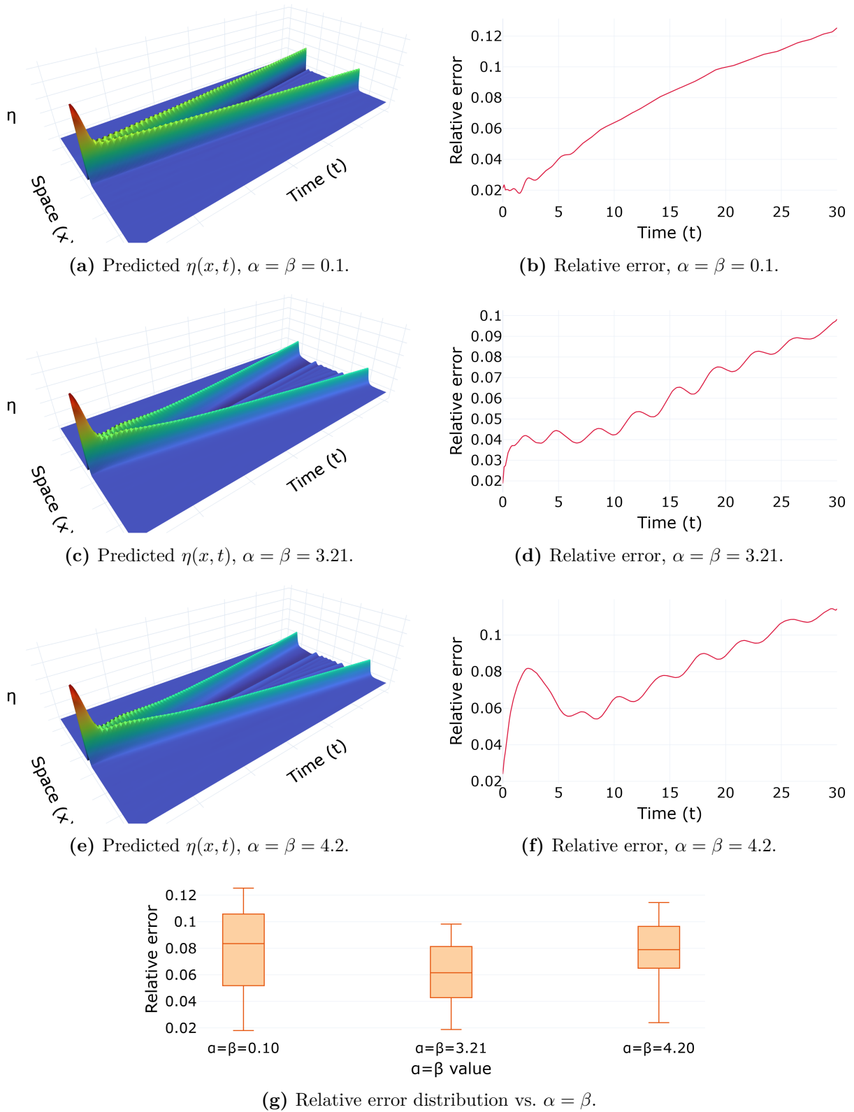
Figure 4.9 – PINO (with data) across the same nonlinearity axis and resolution. The predicted surfaces are visually indistinguishable from the FNO, but the terminal-time spike of Figure 4.8 is absent: the error rises only gently toward t = 30 . The physics residual and initial-condition term act as a temporal regularizer.
