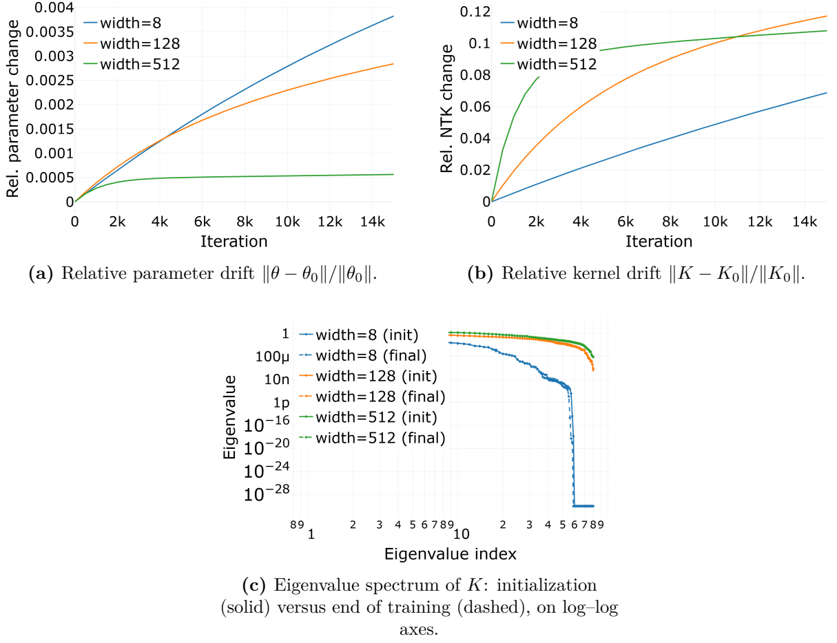
Figure 4.1 – Neural Tangent Kernel diagnostic for the Boussinesq PINN residual at \alpha = \beta = 3.21 , for widths 8, 128 and 512.
