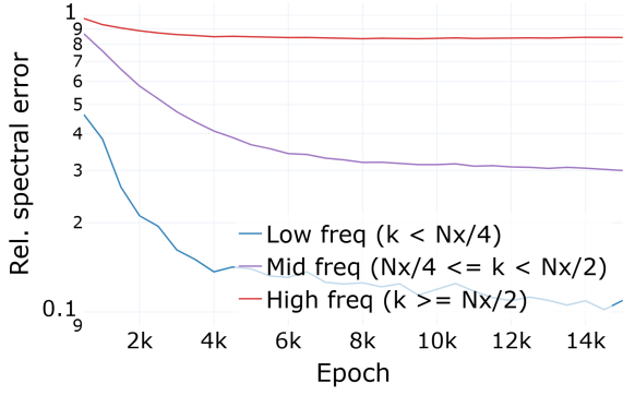
(c) PINO (no data), at \alpha = \beta = 0.1 .
