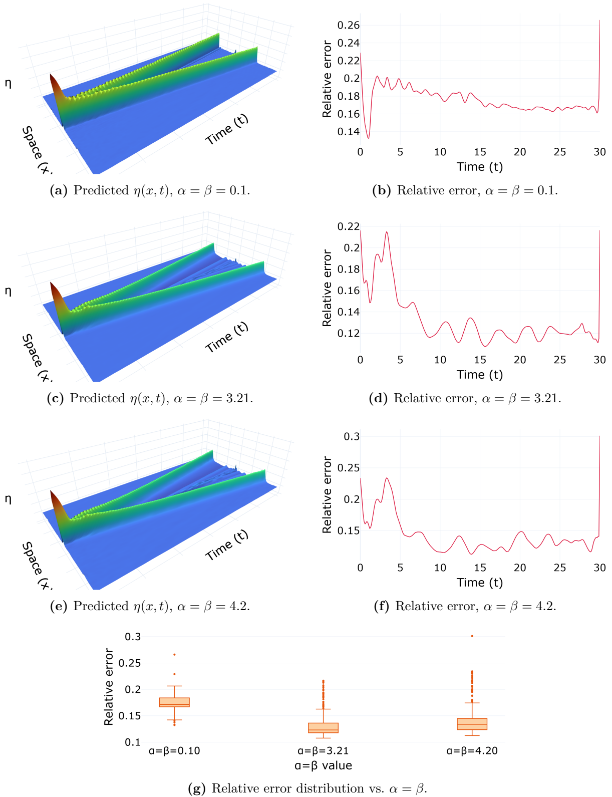
Figure 4.8 – FNO across the nonlinearity axis ( \alpha = \beta \in \{0.1, 3.21, 4.2\} ), evaluated at resolution 256. The predicted surfaces (left) capture the two counter-propagating pulses, but the time-resolved relative error (right) exhibits a pronounced spike at the final time t = 30 : the temporal Gibbs artifact from treating time as a periodic axis.
