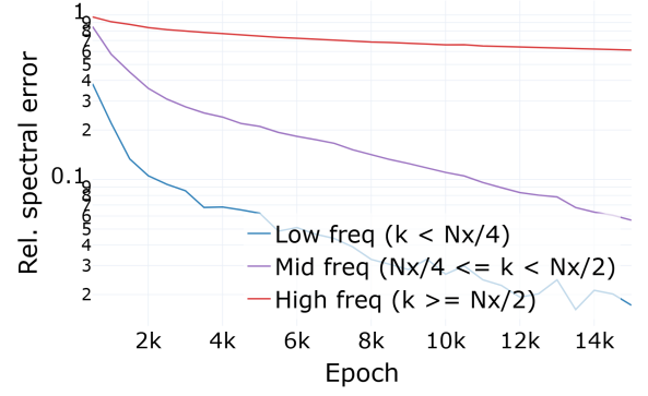
(d) PINO (with data), at \alpha = \beta = 0.1 .
