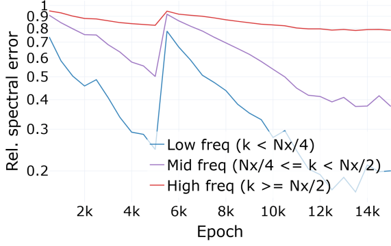
(a) PINN (no data), at \alpha = \beta = 3.21 .
