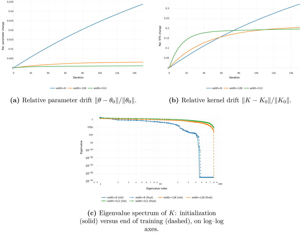
Figure 4.2 – Neural Tangent Kernel diagnostic for the Boussinesq PINN residual at \alpha = \beta = 3.21 , for widths 8, 128 and 512.
