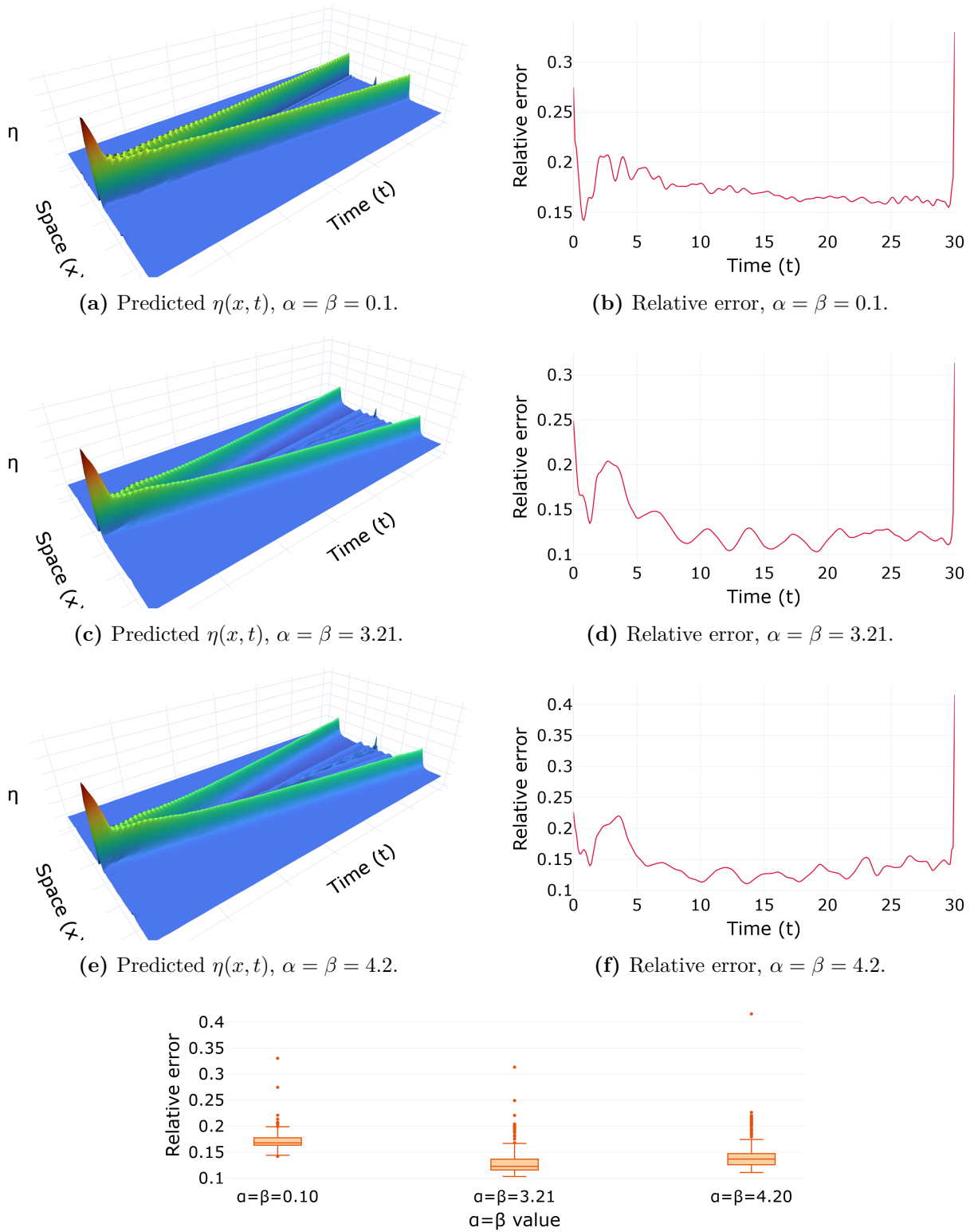
Figure 4.10 – FNO across the nonlinearity axis ( \alpha = \beta \in \{0.1, 3.21, 4.2\} ), evaluated at resolution 256. The predicted surfaces (left) capture the two counter-propagating pulses, but the time-resolved relative error (right) spikes sharply at the final time t = 30 : the temporal Gibbs artifact of treating time as a periodic axis.
