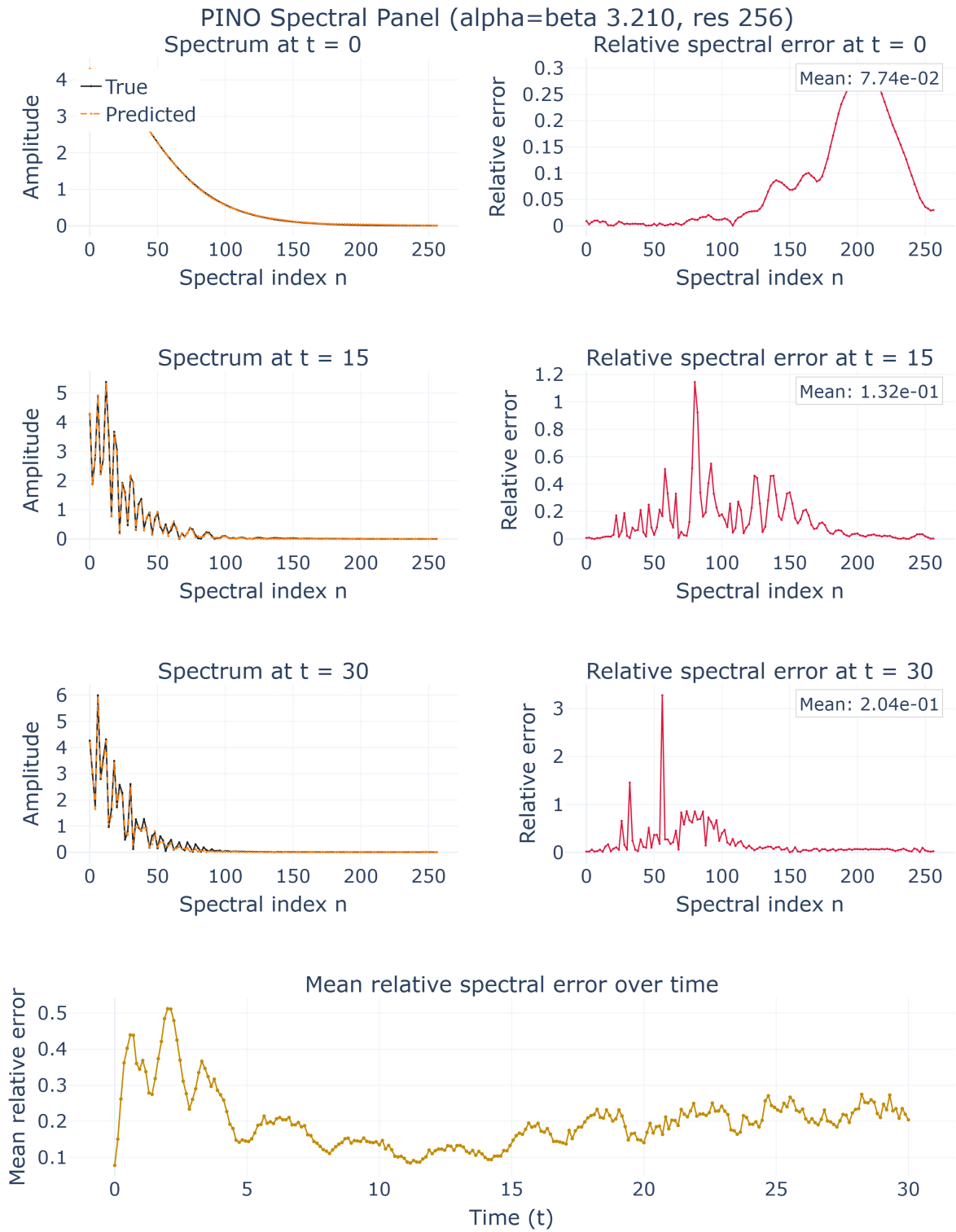
Figure 4.6 – PINO (with data) spatial spectrum at \alpha = \beta = 3.21 . The prediction tracks the reference across the band and, unlike the FNO, the mean error remains bounded in time ( 0.077 \rightarrow 0.13 \rightarrow 0.20 ): the physics residual stabilizes the temporal evolution.
