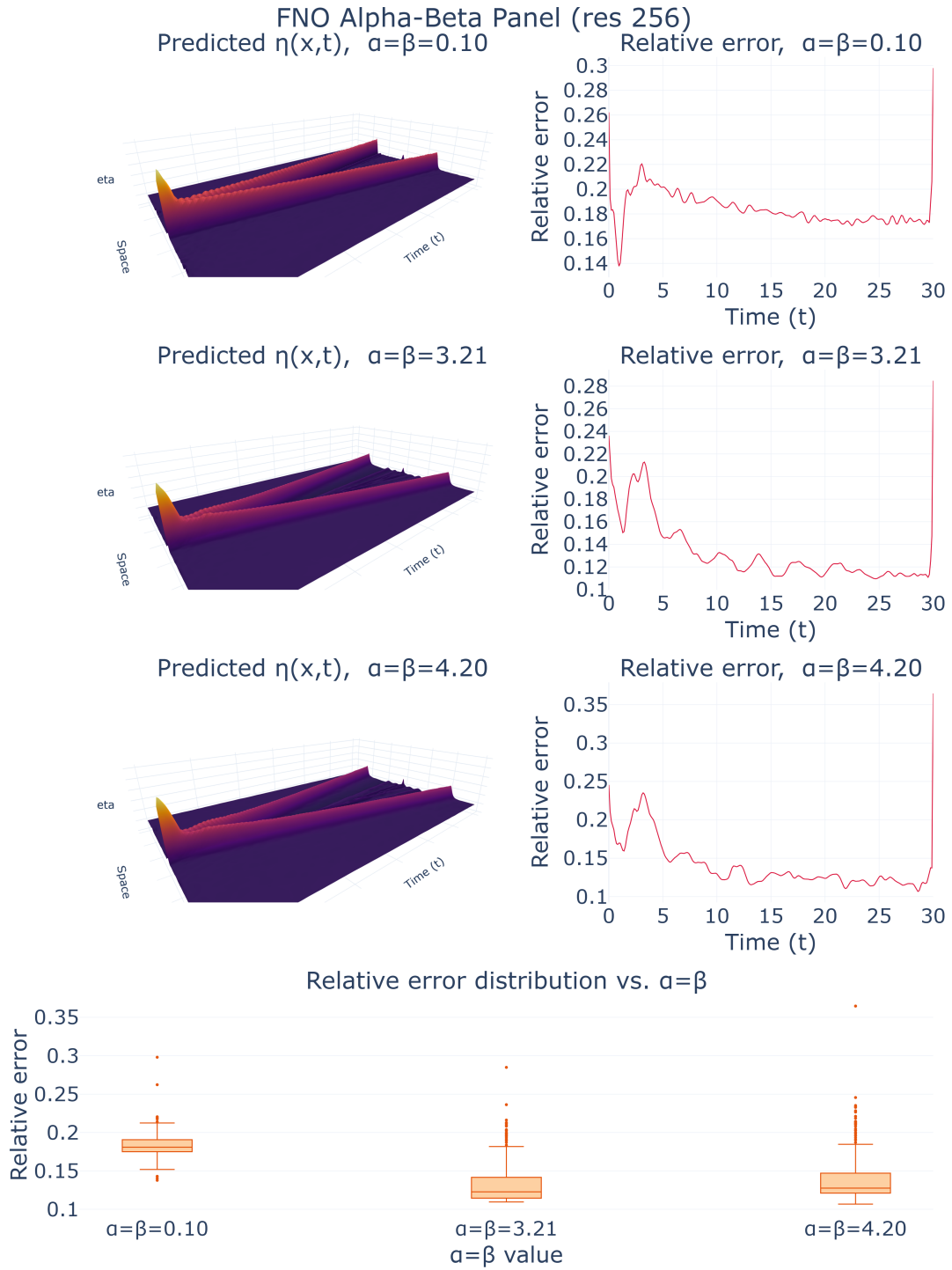
Figure 4.8 – FNO across the nonlinearity axis ( \alpha = \beta \in \{0.1, 3.21, 4.2\} ), evaluated at resolution 256. The predicted surfaces (left) capture the two counter-propagating pulses, but the time-resolved relative error (right) exhibits a pronounced spike at the final time t = 30 : the temporal Gibbs artifact from treating time as a periodic axis.
