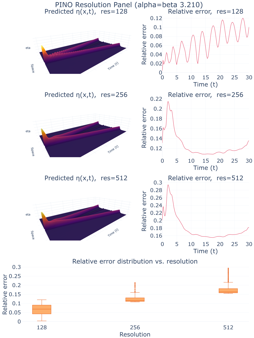
Figure 4.10 – PINO (with data) queried zero-shot at resolutions 128, 256 and 512 at \alpha = \beta = 3.21 . The operator produces a coherent field at every resolution, but the relative error against the pseudospectral reference grows with resolution (median error rising from about 0.07 at 128 to about 0.16 at 512): discretization-invariance of form is not accuracy-invariance.
