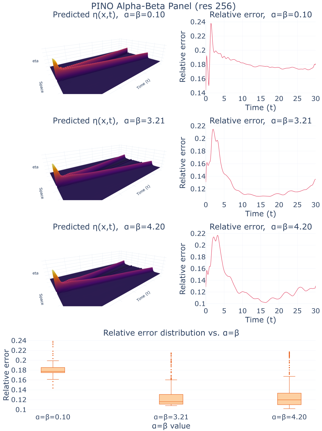
Figure 4.9 – PINO (with data) across the same nonlinearity axis and resolution. The predicted surfaces are visually indistinguishable from the FNO, but the terminal-time spike of Figure 4.8 is absent: the error rises only gently toward t = 30 . The physics residual and initial-condition term act as a temporal regularizer.
