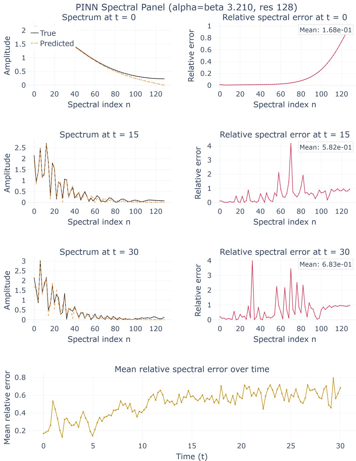
Figure 4.4 – PINN (with data) spatial spectrum at \alpha = \beta = 3.21 . The low-wavenumber crests are tracked more closely than in Figure 4.3, but the high-wavenumber undershoot and the growth of the mean error in time ( 0.17 \rightarrow 0.58 \rightarrow 0.68 ) persist.
