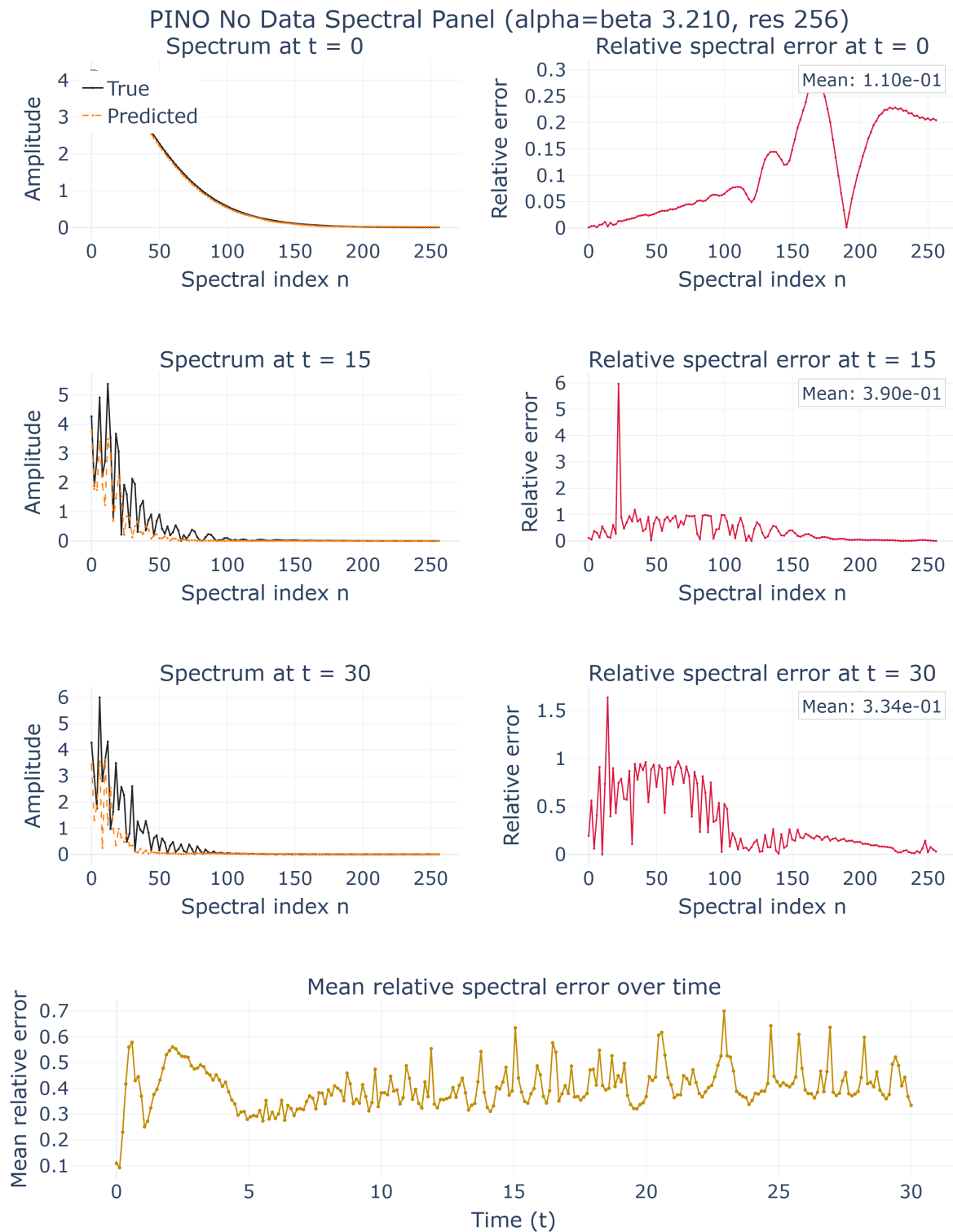
Figure 4.7 – PINO (no data) spatial spectrum at \alpha = \beta = 3.21 . Without the supervised term the low- and mid-band undershoot returns (mean error 0.11 \rightarrow 0.39 \rightarrow 0.33 ), confirming that the physics residual alone does not overcome spectral bias.
