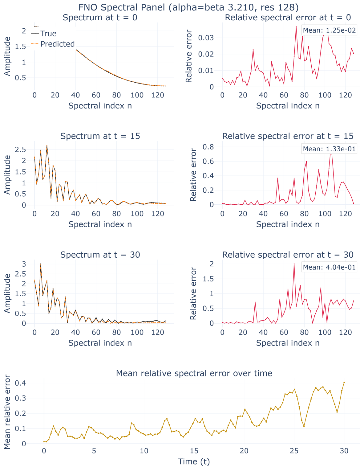
Figure 4.5 – FNO spatial spectrum at \alpha = \beta = 3.21 . Low and mid wavenumbers are tracked almost exactly (mean error 0.013 at t = 0 ), but the error migrates to the high modes and grows steadily in time, reaching a mean of 0.40 at t = 30 .
