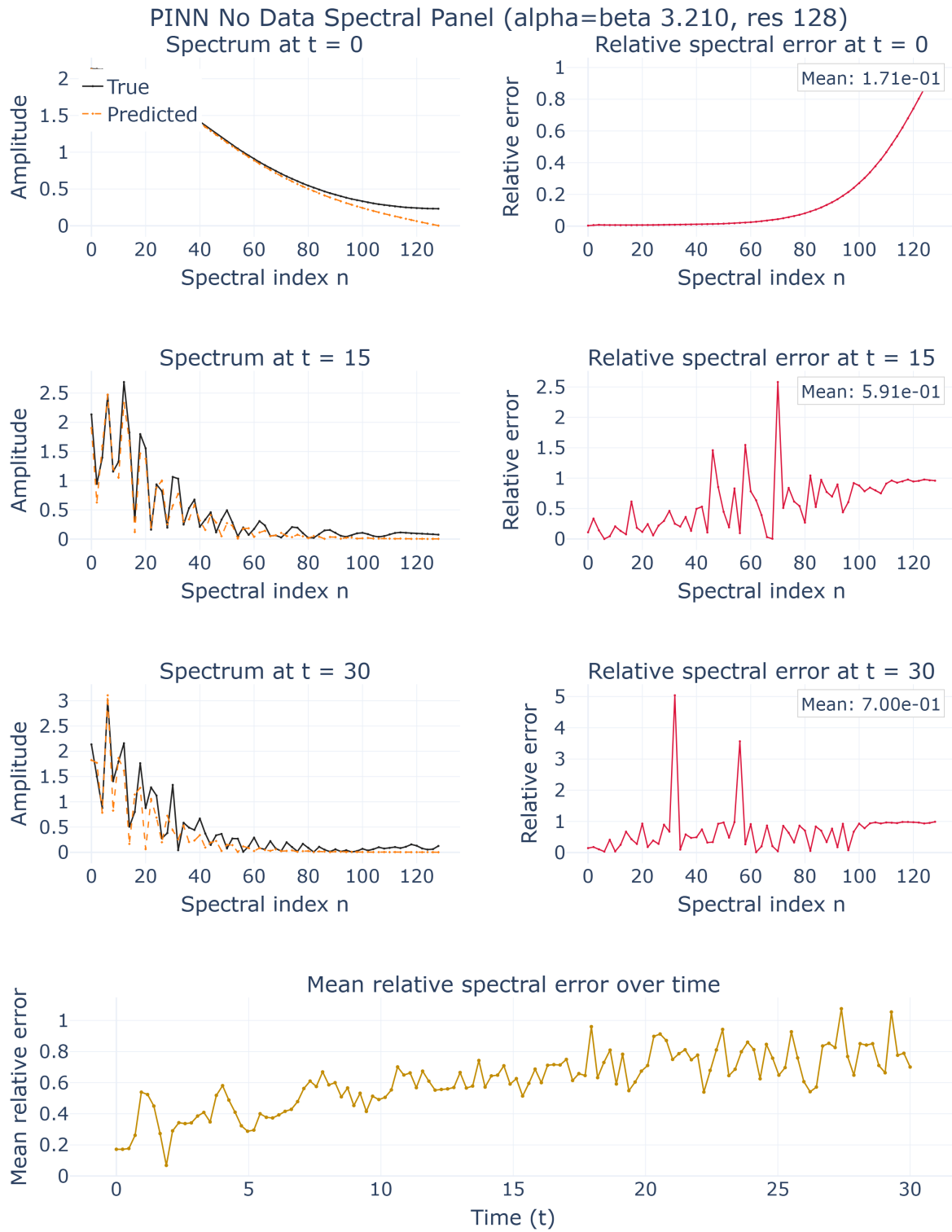
Figure 4.3 – PINN (no data) spatial spectrum at \alpha = \beta = 3.21 . Already at t = 0 the predicted spectrum undershoots the reference tail, and the relative error rises monotonically with wavenumber; the mean spectral error grows from 0.17 at t = 0 to 0.70 at t = 30 .
