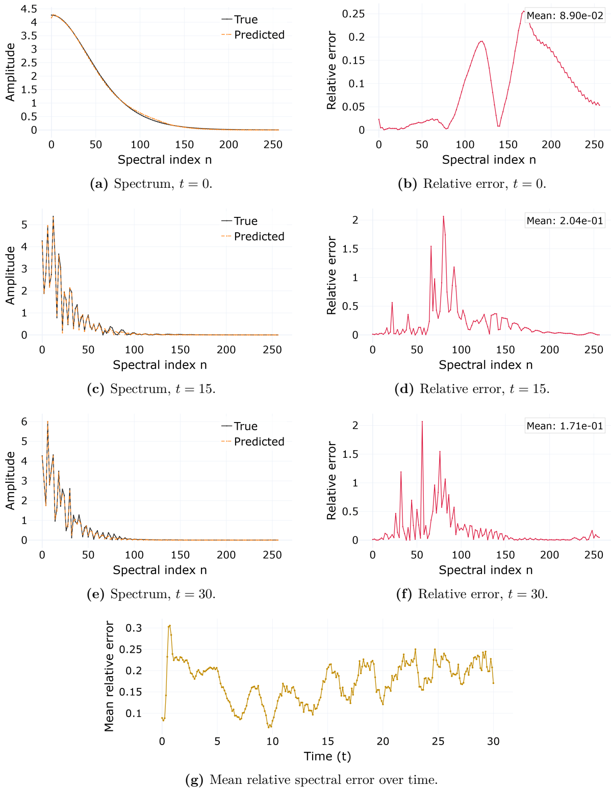
Figure 4.8 – PINO (with data) spatial spectrum at \alpha = \beta = 3.21 . The prediction tracks the reference across the band and, unlike the FNO, the mean error does not blow up at late time: it rises to 0.20 at t = 15 and settles to 0.17 at t = 30 ( 0.09 \rightarrow 0.20 \rightarrow 0.17 ). The physics residual steadies the temporal evolution.
