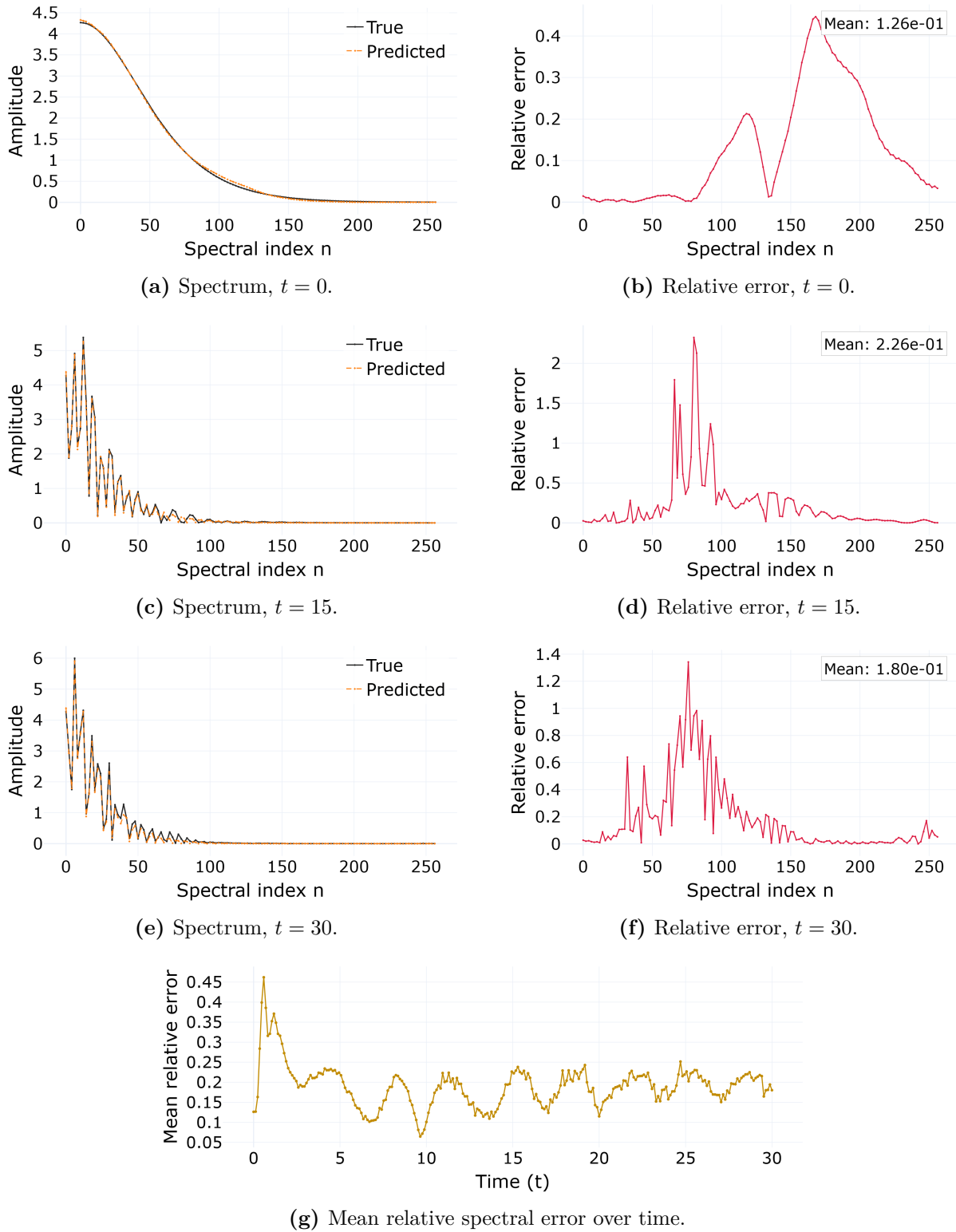
Figure 4.9 – PINO (no data) spatial spectrum at \alpha = \beta = 3.21 . Without the supervised term the low- and mid-band undershoot returns (mean error 0.13 \rightarrow 0.23 \rightarrow 0.18 ), confirming that the physics residual alone does not overcome spectral bias.
