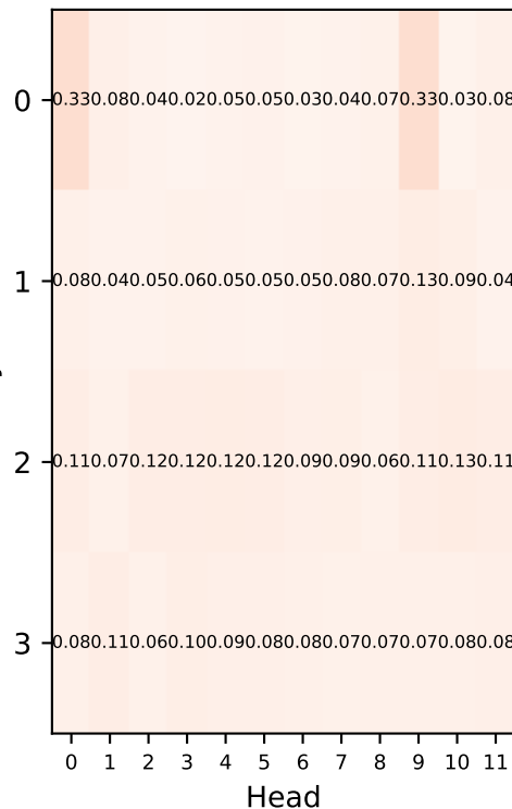
BiMGA Uniform MRR=0.313 | Mean KL=0.086
