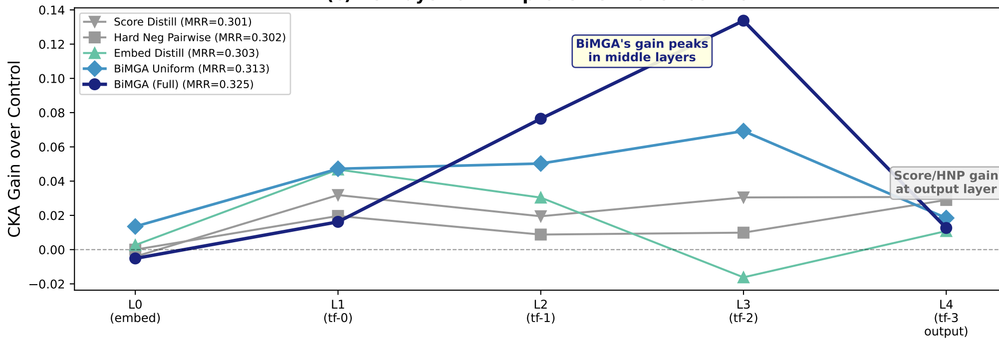
(c) Per-layer CKA improvement over Control
