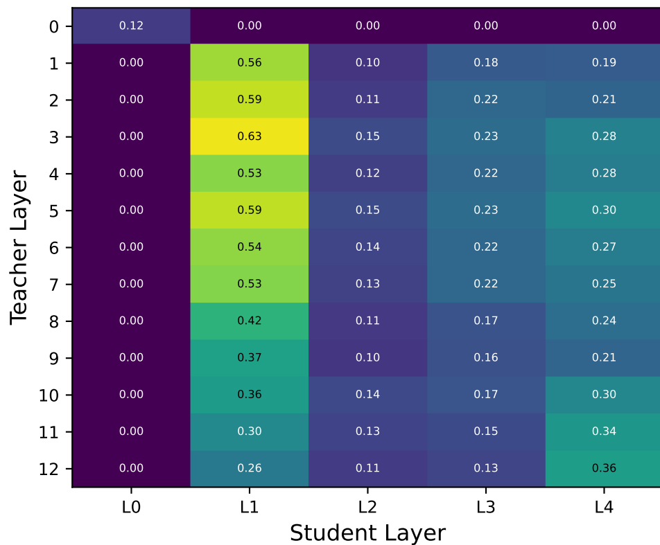
(a) Control (Supervised) MRR = 0.205
