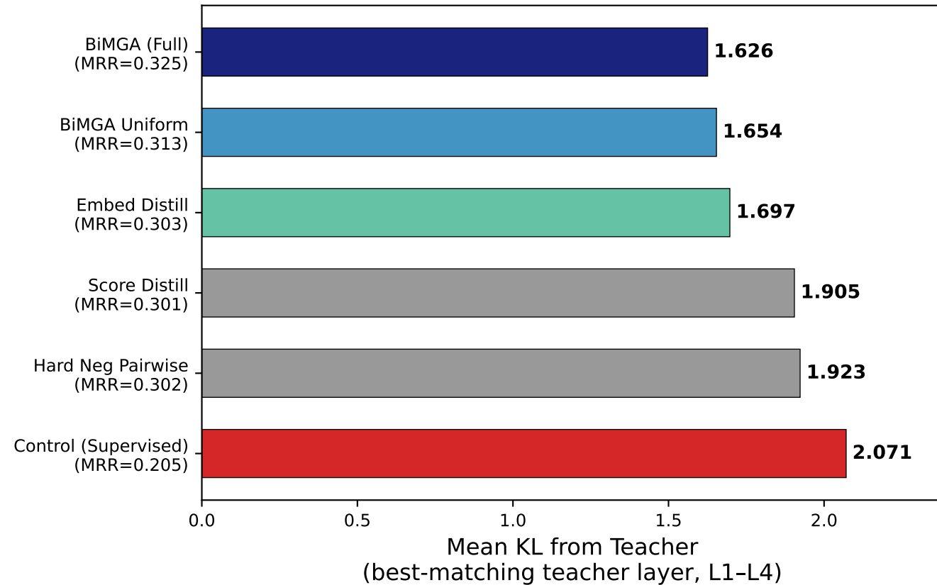
(a) Overall Attention Similarity to Teacher
