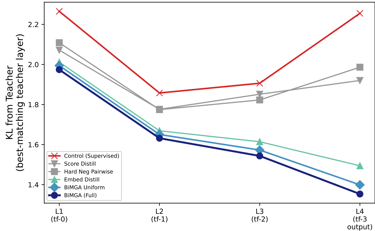
(b) Per-layer Attention Divergence from Teacher
