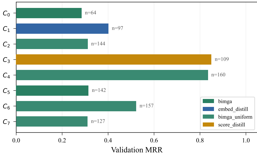
(b) Per-Cluster Best Model Assignment (k = 8)
