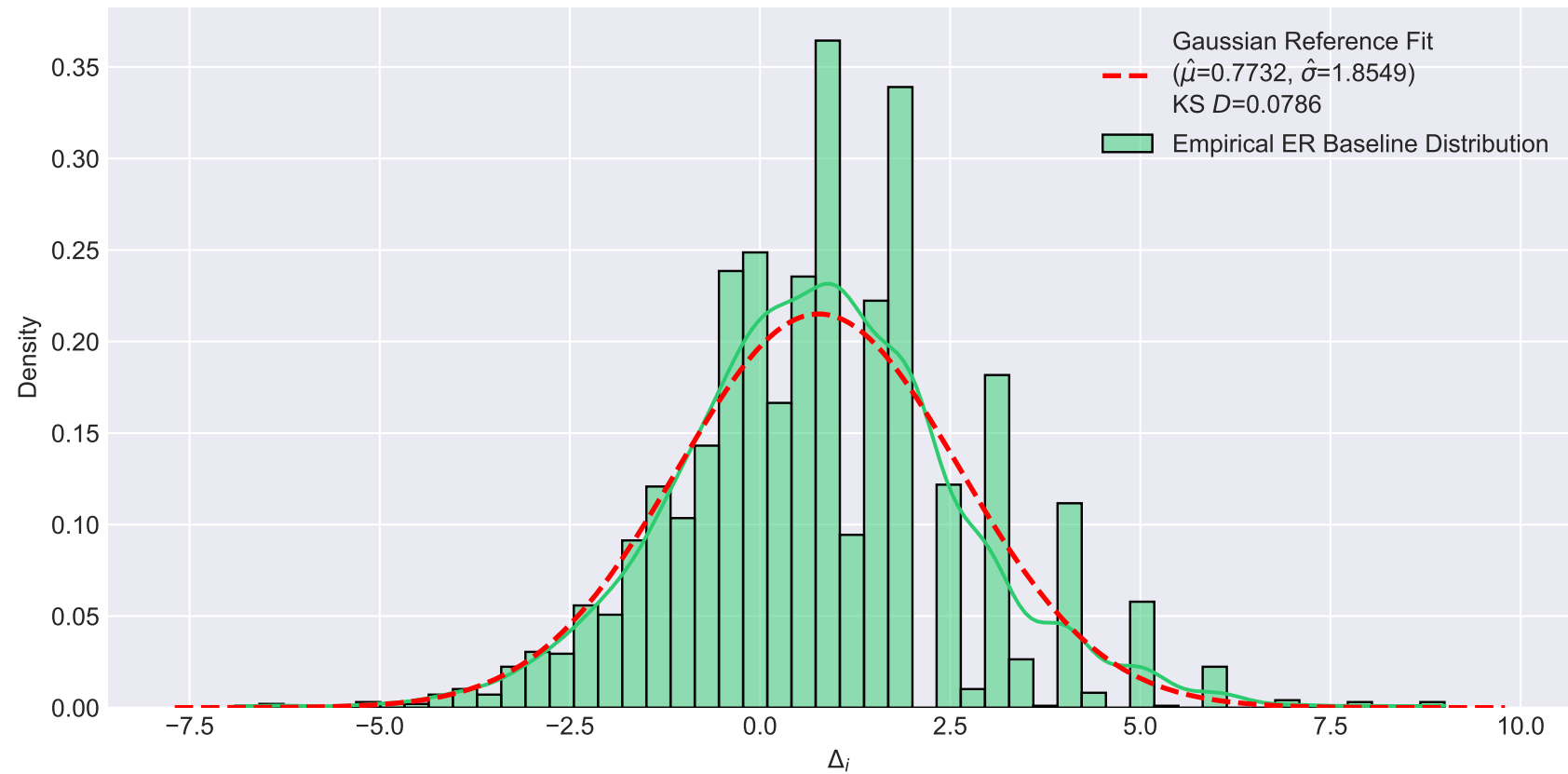
Empirical ER Baseline Distribution vs. Gaussian Model of \Delta_i (CiteSeer - Degree Centrality)
