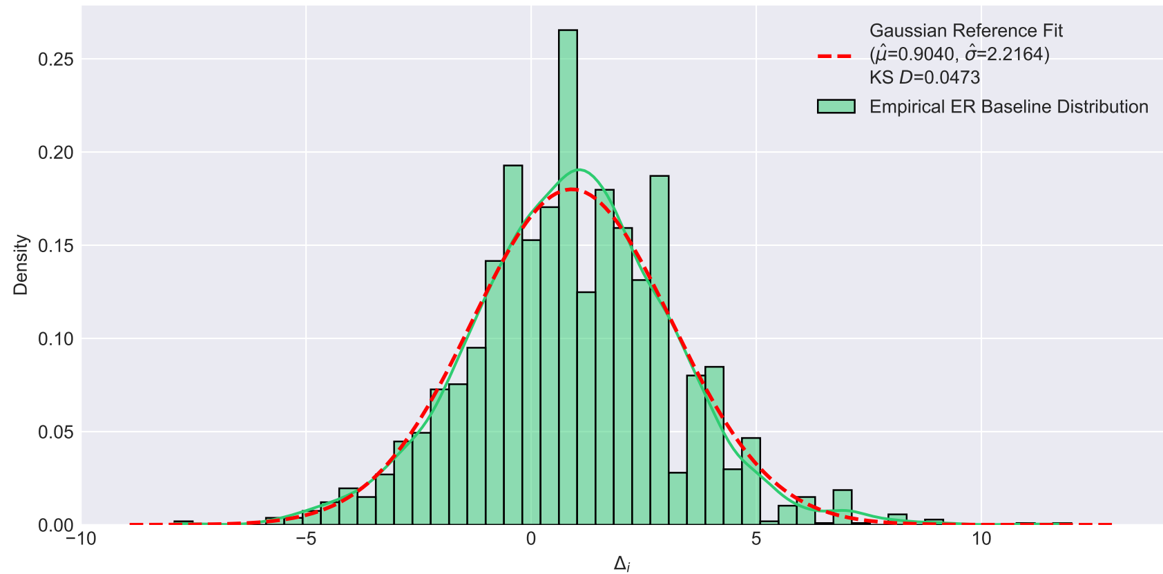
Empirical ER Baseline Distribution vs. Gaussian Model of \Delta_i (Cora - Degree Centrality)
