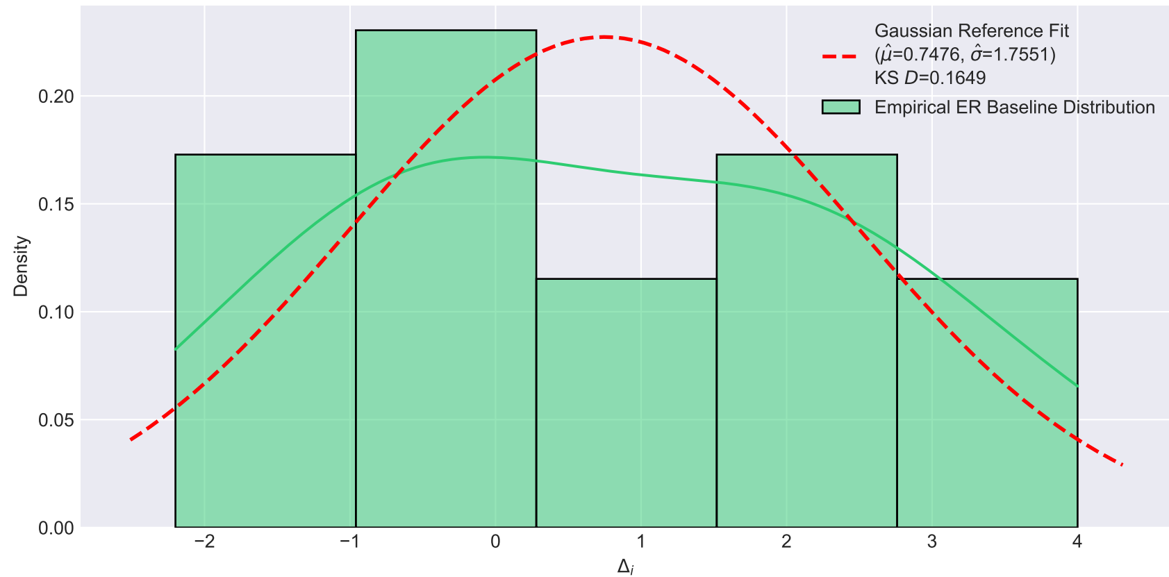
Empirical ER Baseline Distribution vs. Gaussian Model of \Delta_i (Florentine Families - Degree Centrality)
