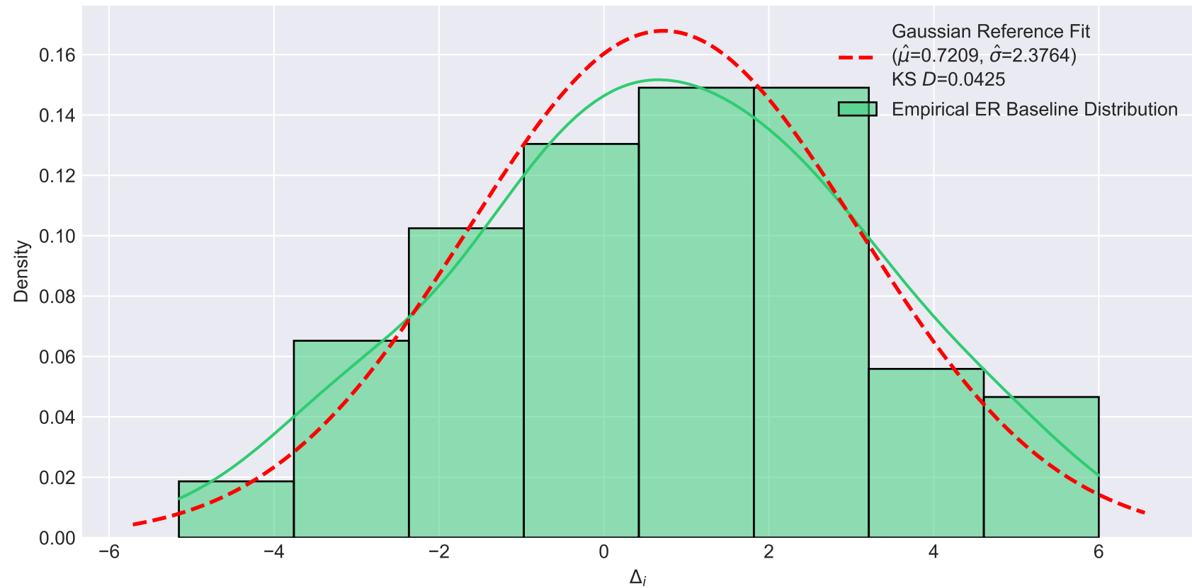
Empirical ER Baseline Distribution vs. Gaussian Model of \Delta_i (Les Miserables - Degree Centrality)
