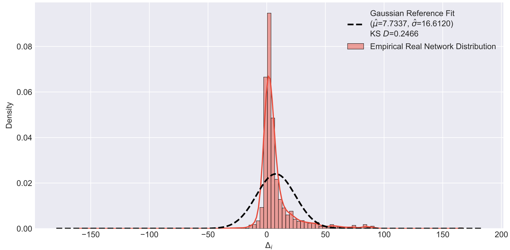
Empirical Real Network Distribution vs. Gaussian Model of \Delta_i (Cora - Degree Centrality)
