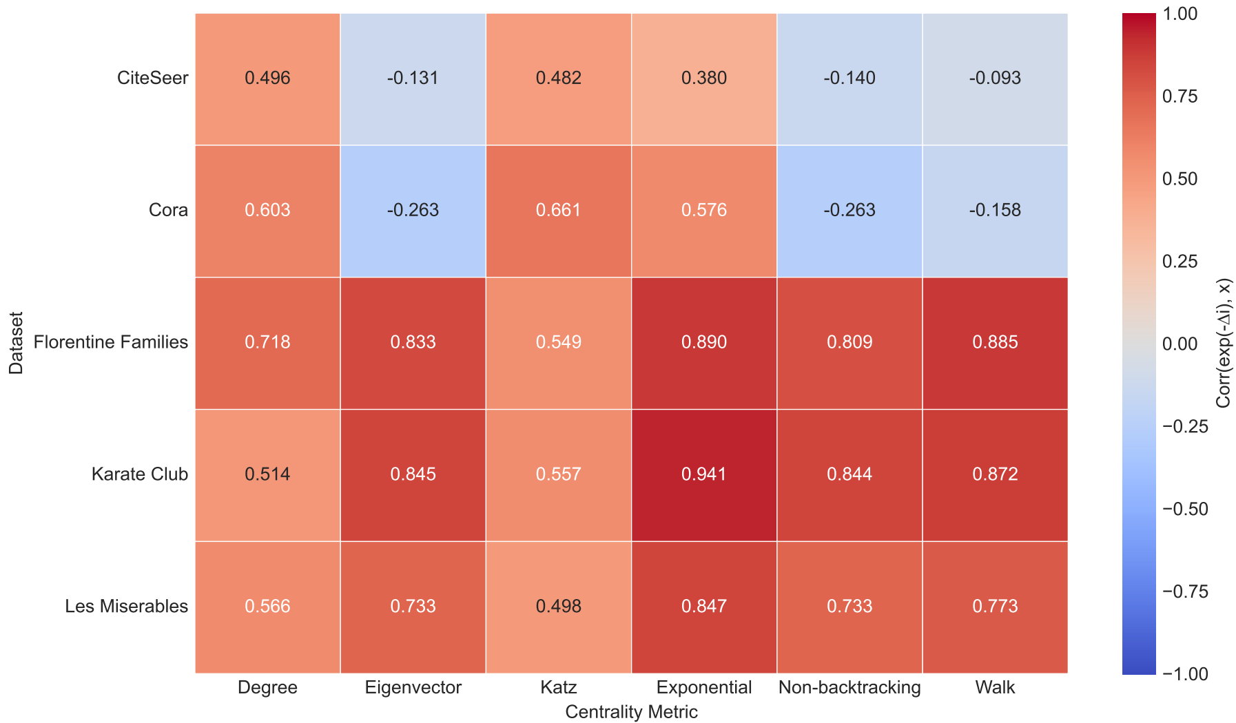
Correlation Heatmap: Classic Centrality Measures vs \exp(-\Delta_i) across Datasets
