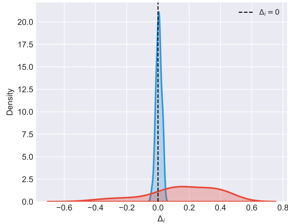
Exponential Centrality
