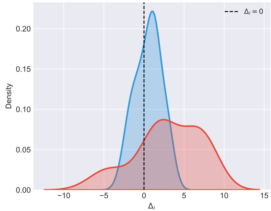
Katz Centrality
