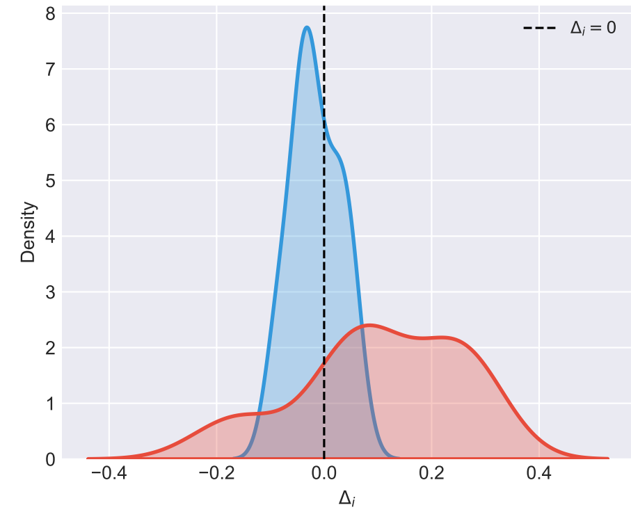
Non-backtracking Centrality
