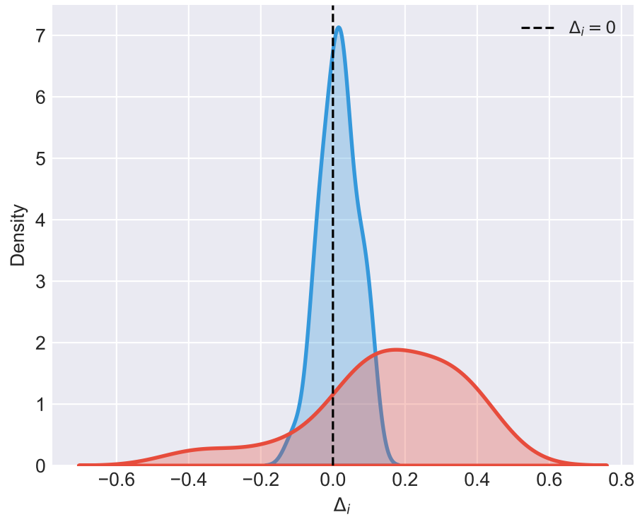
Katz Centrality
