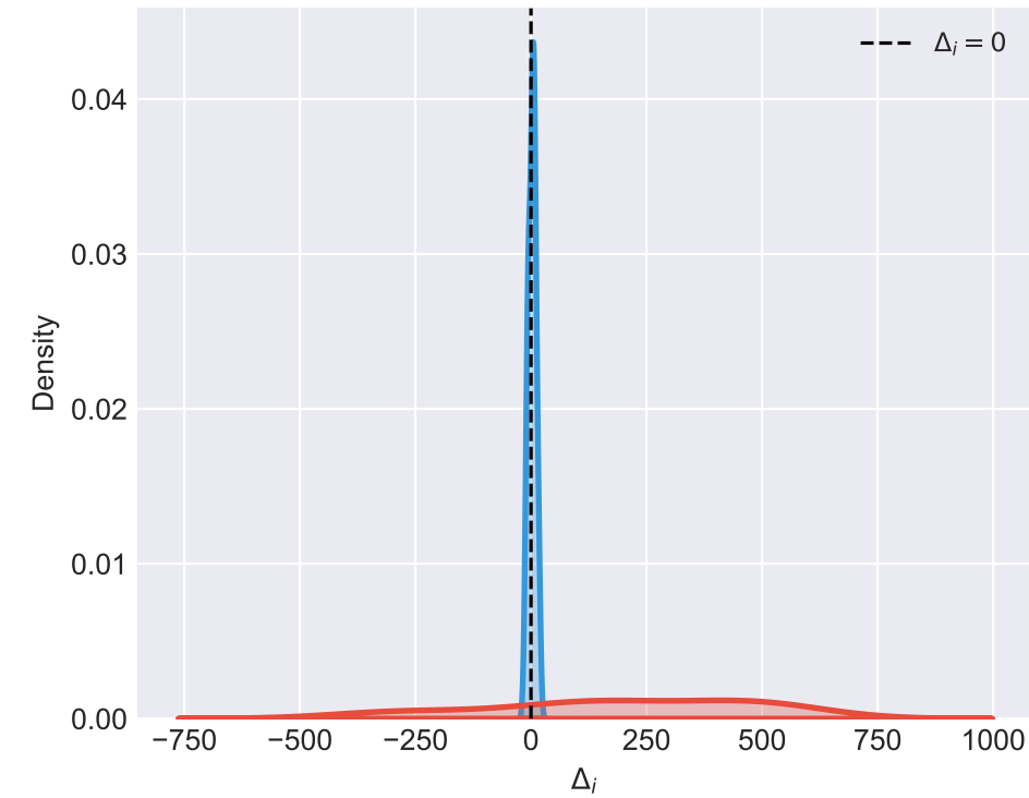
Non-backtracking Centrality
