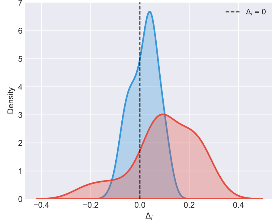
Exponential Centrality
