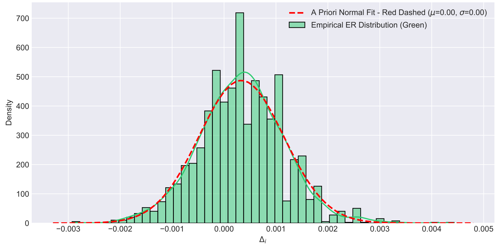
Empirical vs A Priori Distribution of \Delta_i (Cora - Degree) (Green = Empirical ER, Red Dashed = Theoretical Normal Fit)
