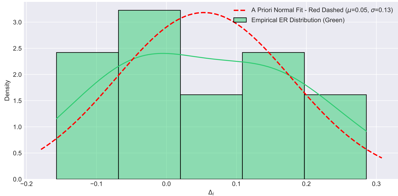
Empirical vs A Priori Distribution of \Delta_i (Dolphins - Degree) (Green = Empirical ER, Red Dashed = Theoretical Normal Fit)
