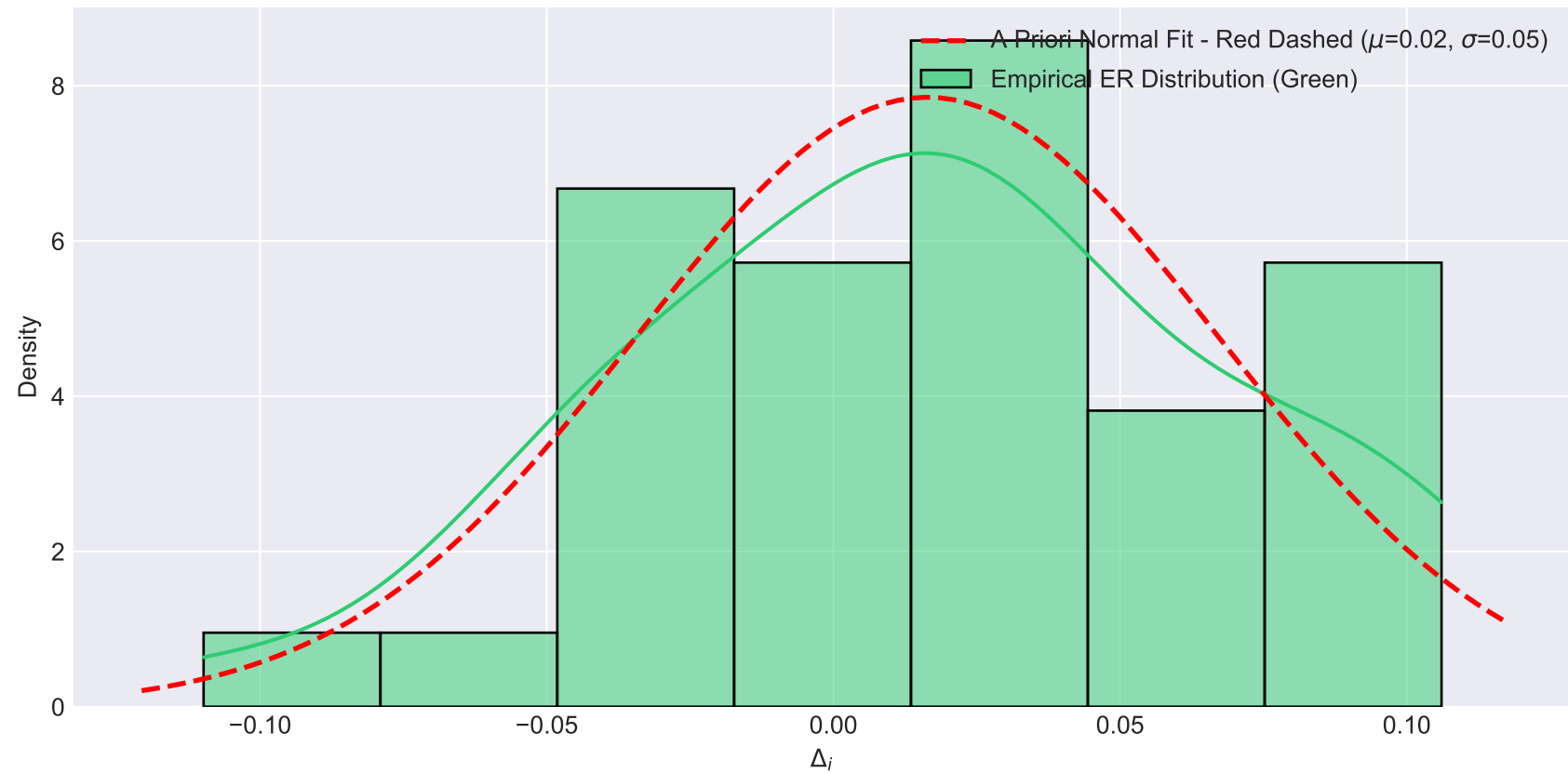
Empirical vs A Priori Distribution of \Delta_i (Karate Club - Degree) (Green = Empirical ER, Red Dashed = Theoretical Normal Fit)
