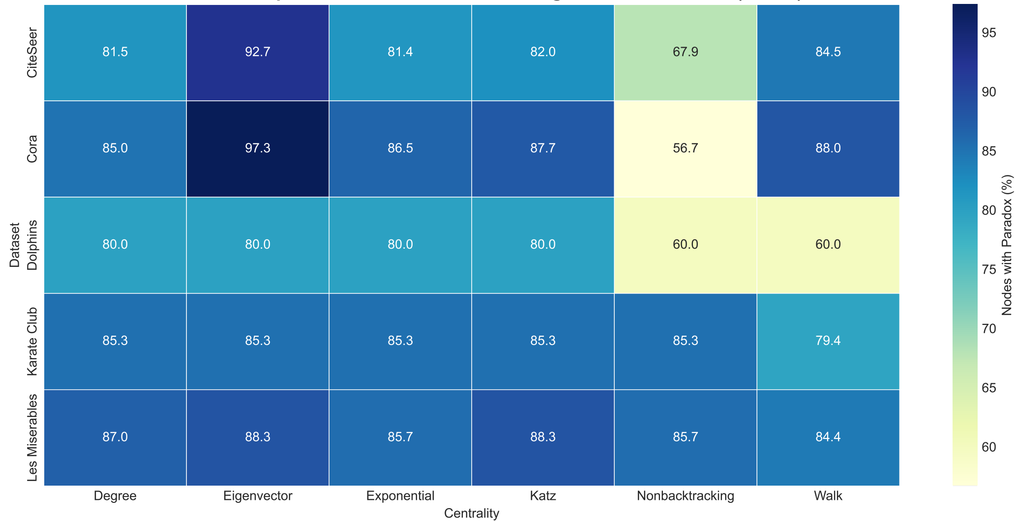
Local Friendship Paradox: % of Nodes with Neighbors More Central ( \Delta \geq 0 )
