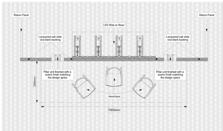
Top / Plan View: Set overview with labels - Scale 1:35
