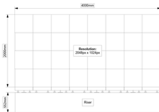
Front View: LED Wall on riser - Scale 1:25 "8x4 (500mm x 500mm Panels)"
