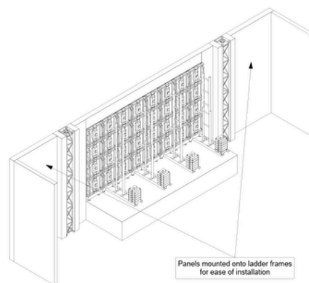
Rear Isometric View: BOH - Scale 1:25
