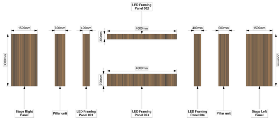
Front View: Panel Construction Layout - Scale 1:50
