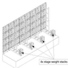
Rear Isometric View: LED Wall on riser - Scale 1:50
