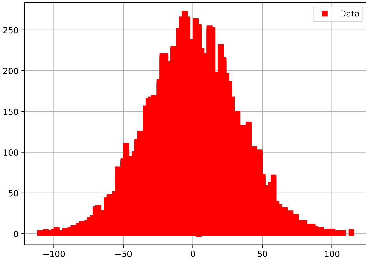
Galton Board result for N = 10000
