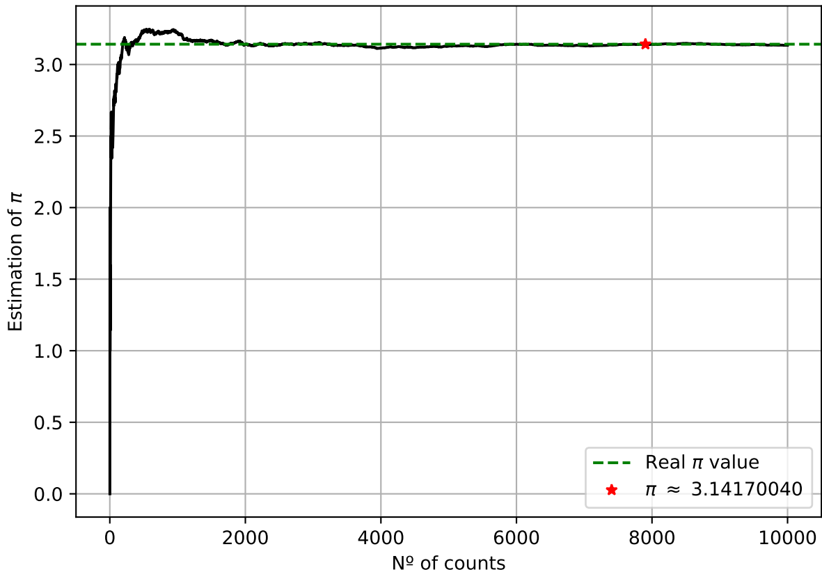
\pi estimation via Monte Carlo algorithm
