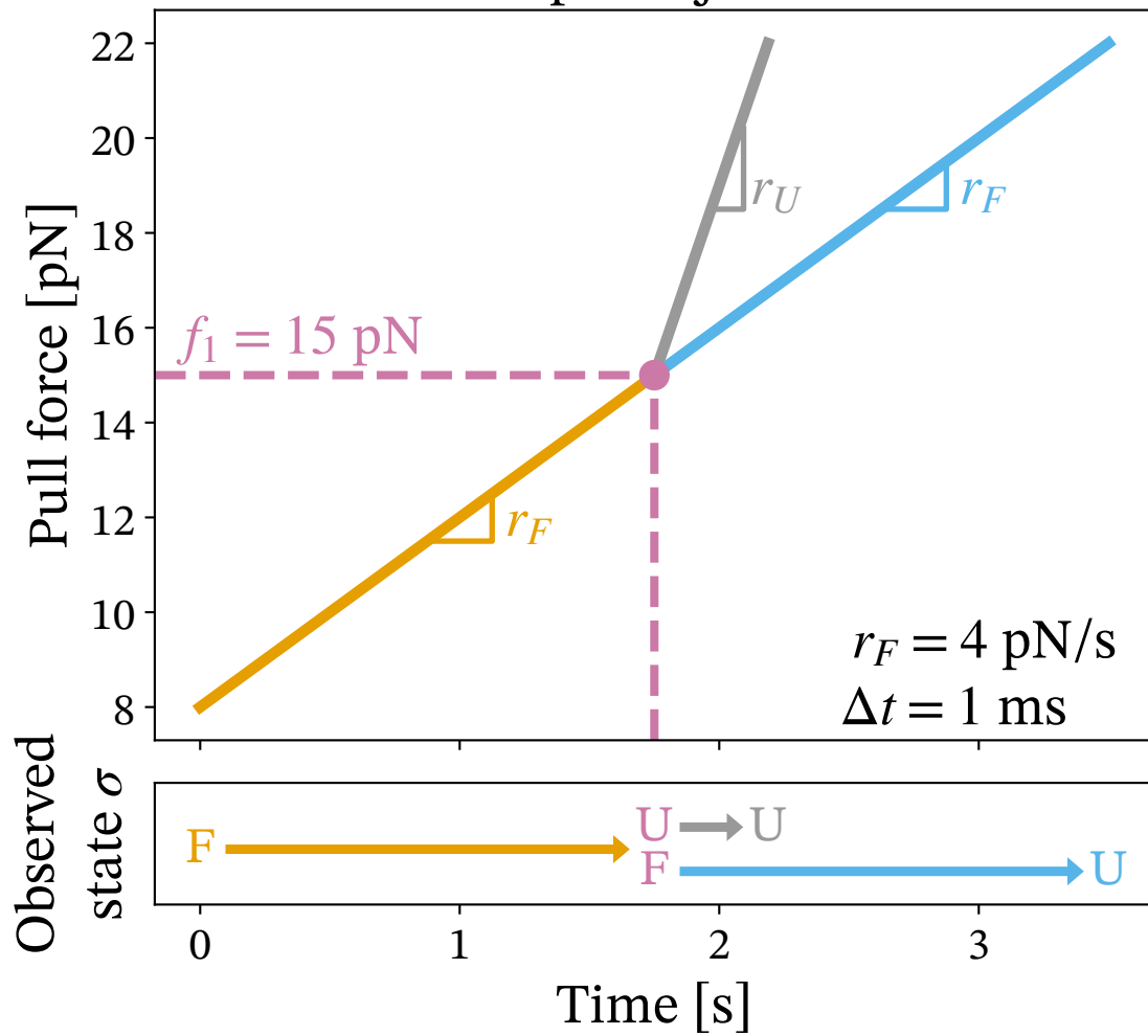
Example trajectories
