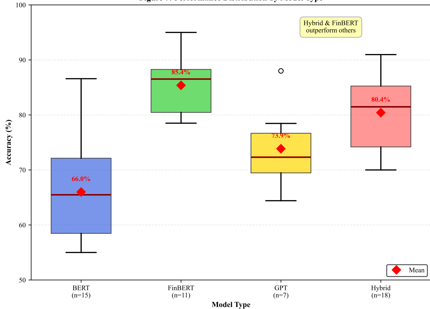
Figure 7: Performance Distribution by Model Type
