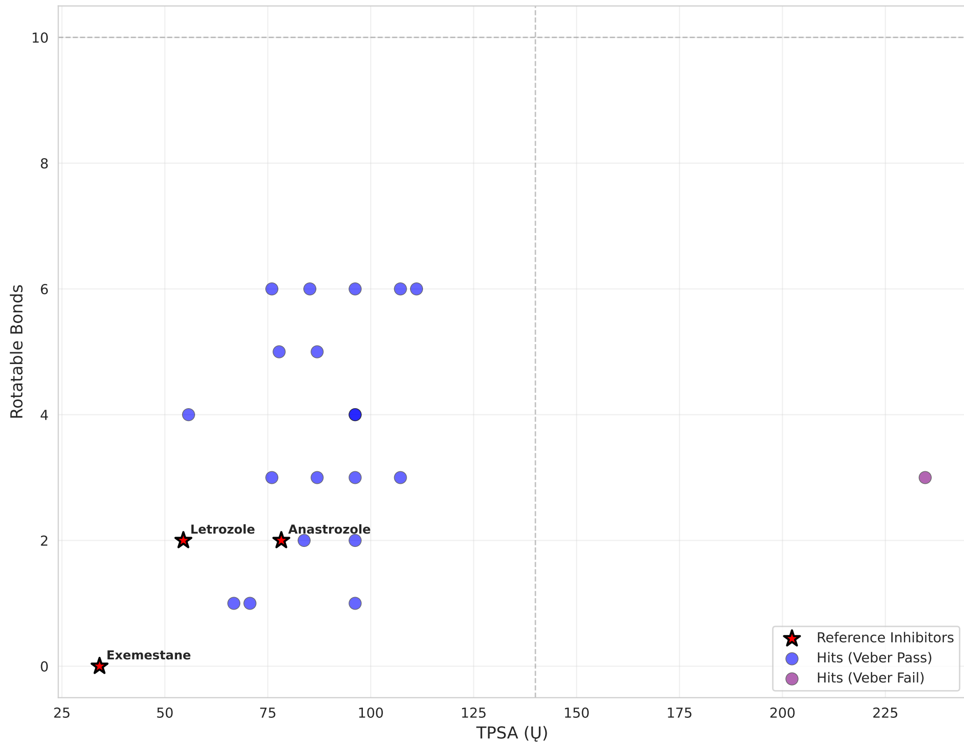
ADMET Profile: TPSA vs Rotatable Bonds
