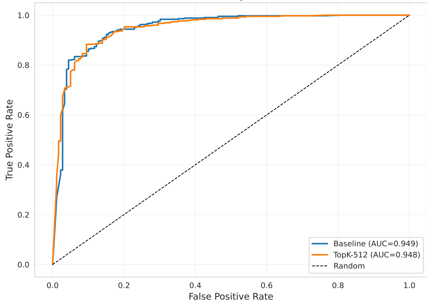
ROC Curve - Binary Classification
