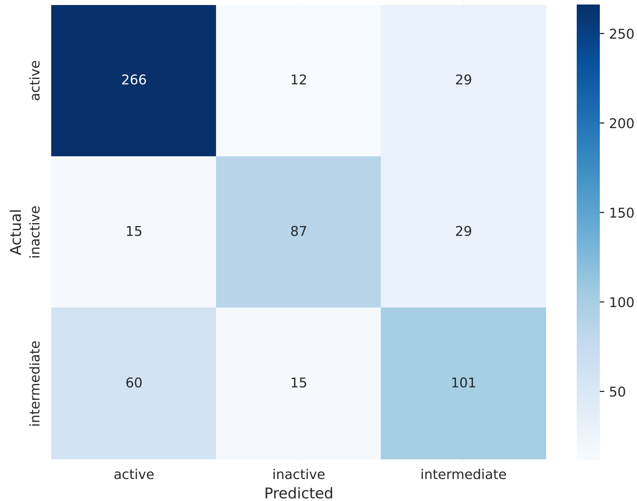
Baseline (2048 features)
