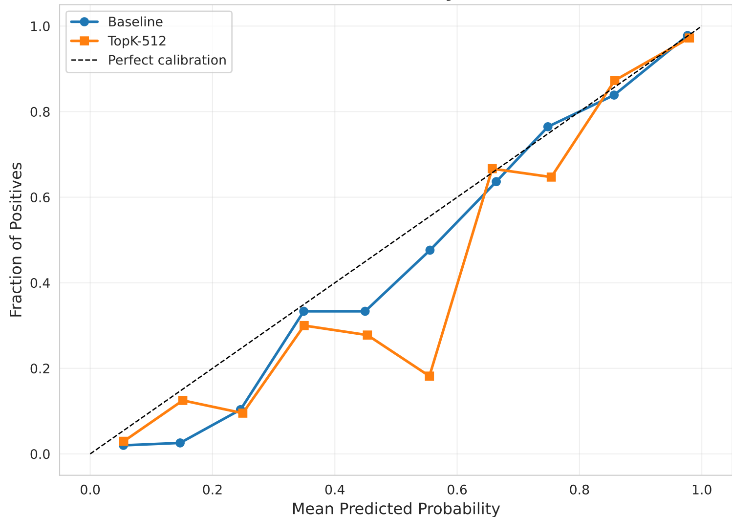
Calibration Curve - Binary Classification
