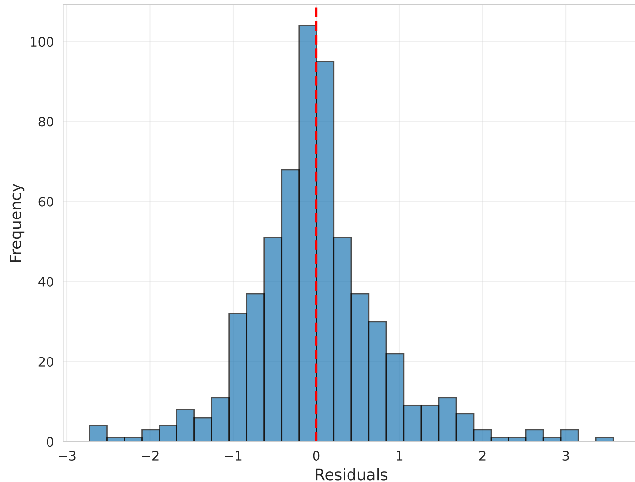
Baseline (MAE=0.569)
